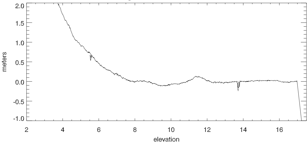
Range - linear fit vs elevation'
