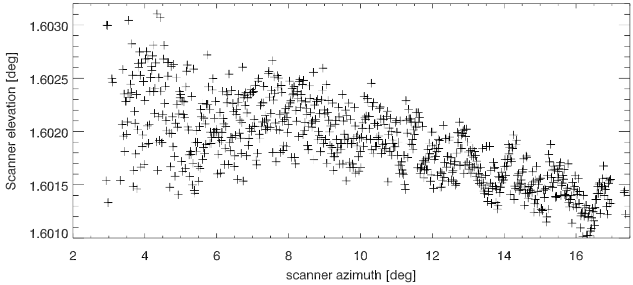
Az vs el postion for az=1.6 elevation strip
