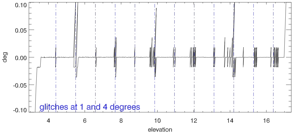
Elevation ramp - linear fit vs elevation
