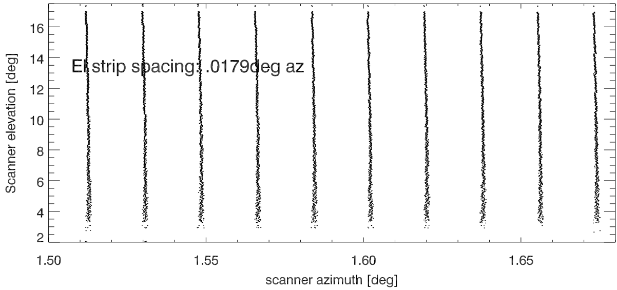
11mar20 P50 scan19(270m Res). az vs el samples for .161 degs of az
