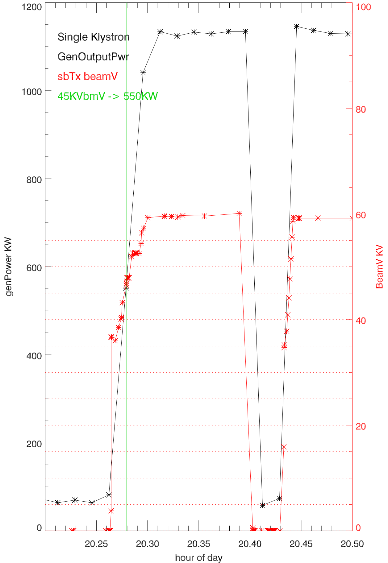
01sep17 sbtx BeamVoltage and generator Power
