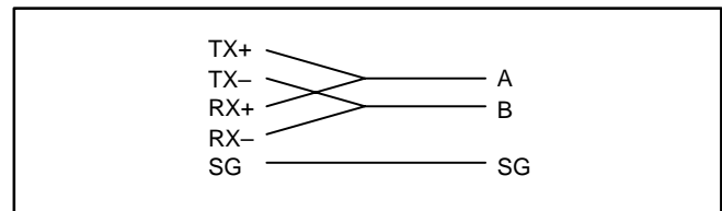
FIGURE 24. CONVERTING THE RS-485 COMMUNICATIONS CABLE
