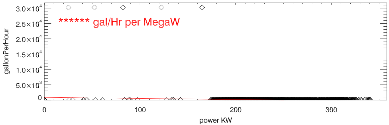
Fuel Rate vs power (sum all generators)
