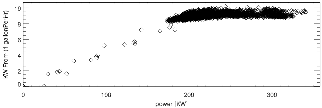
Efficiency: KW for 1 gallon/hour. (sum all generators)
