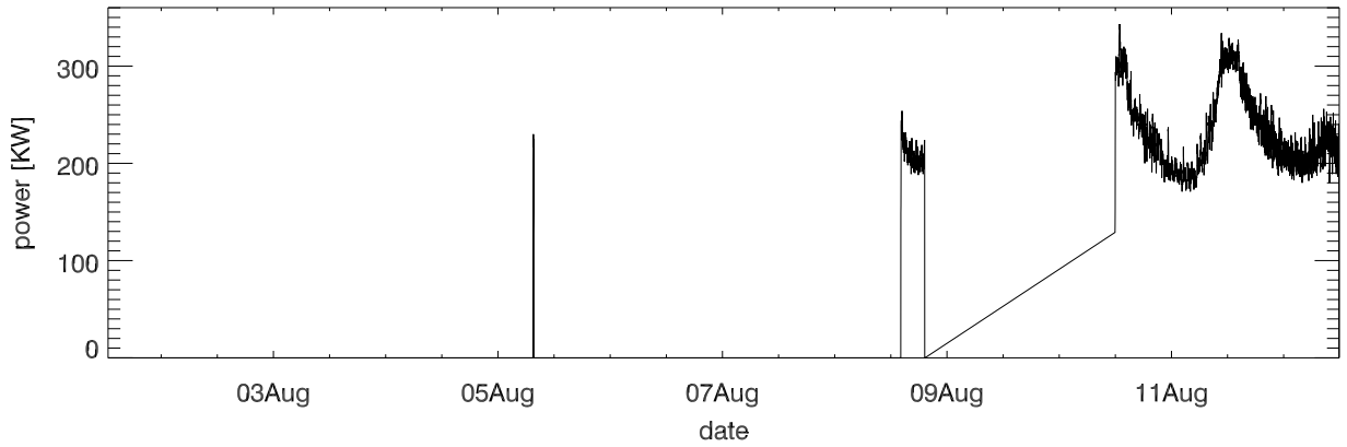
Total power vs Time (sum all generators)
