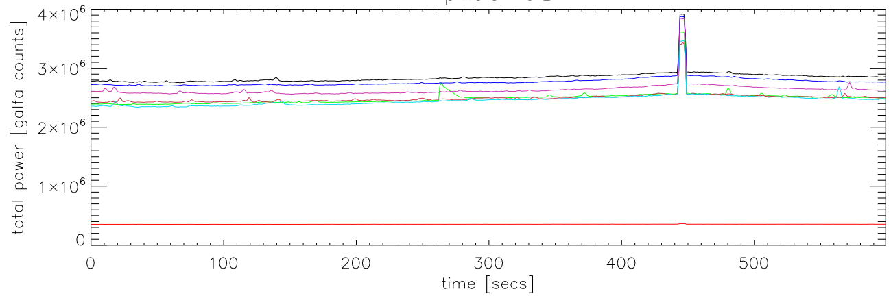
13jul05 a2004 galfa file:.0008 total pwr vs time Pixel 2 Narrow band
