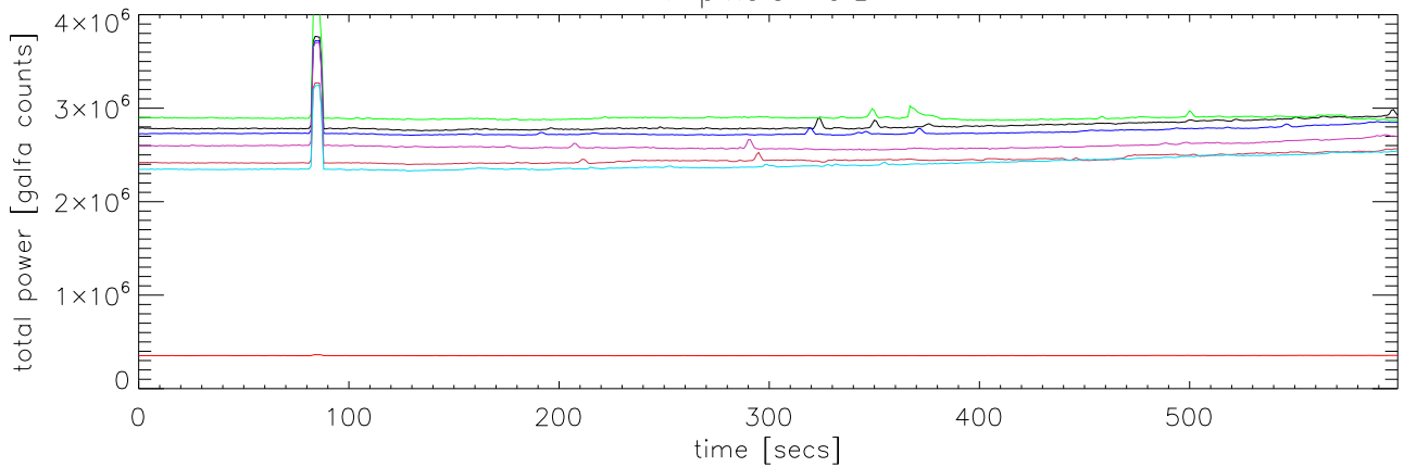
13jul05 a2004 galfa file:.0006 total pwr vs time Pixel 2 Narrow band
