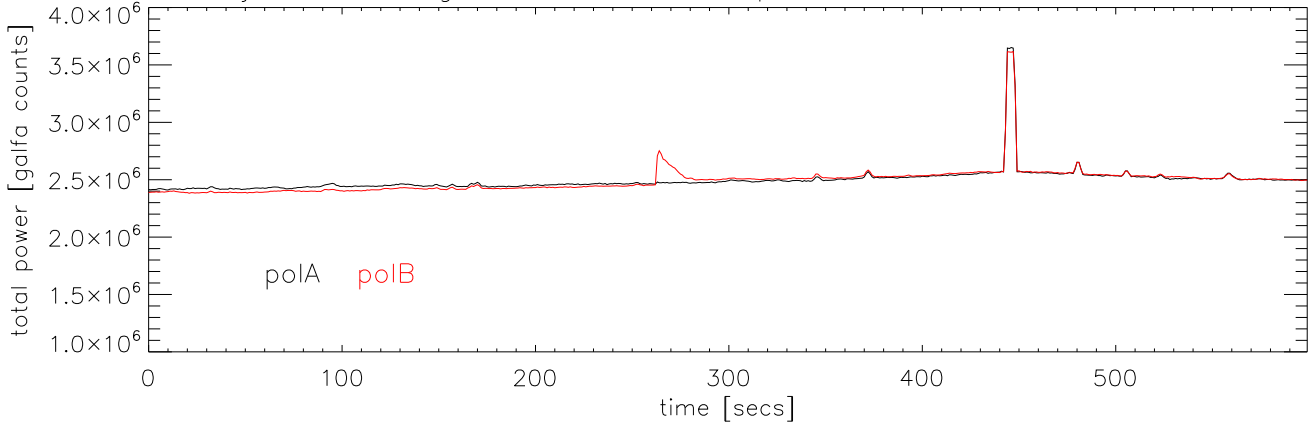
13jul05 a2004 galfa file:.0008 total pwr vs time Pixel 2 Wide band
