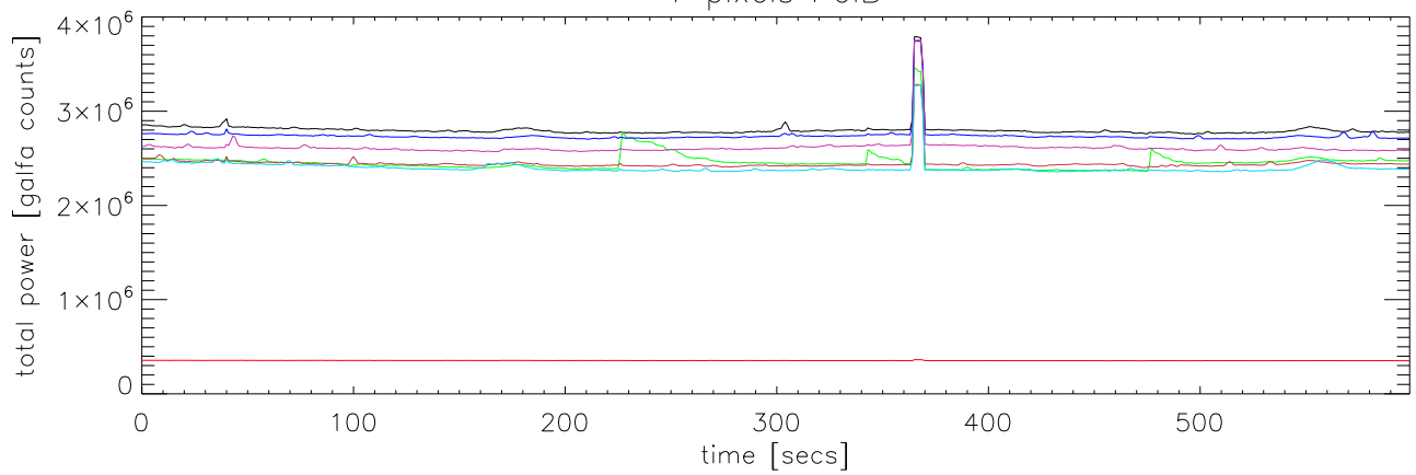
13jul05 a2004 galfa file:.0009 total pwr vs time Pixel 2 Narrow band
