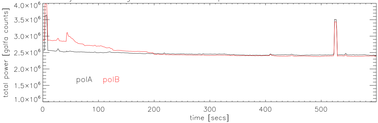
13jul05 a2004 galfa file:.0007 total pwr vs time Pixel 2 Wide band
