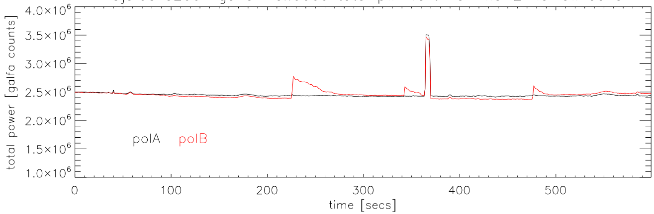
13jul05 a2004 galfa file:.0009 total pwr vs time Pixel 2 Wide band
