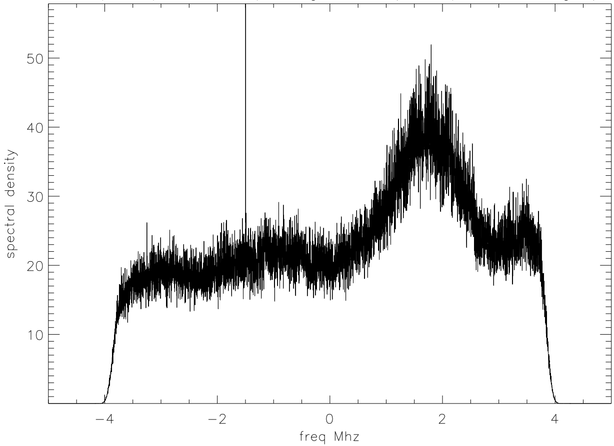
07sep05 spectra of clp height data (100 spectra averaged)
