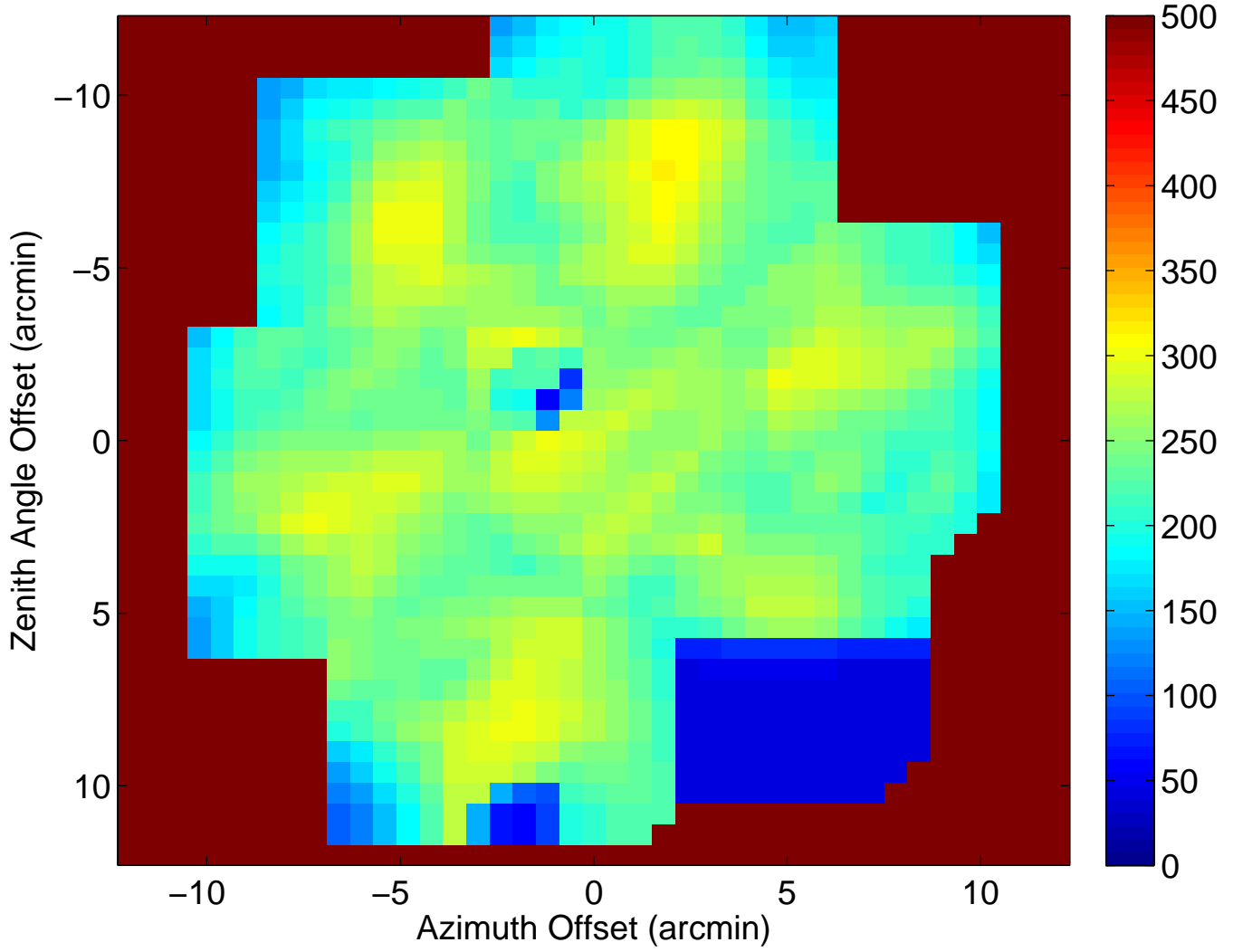
Ae/Tsys Map ( z = 19.965 cm)
