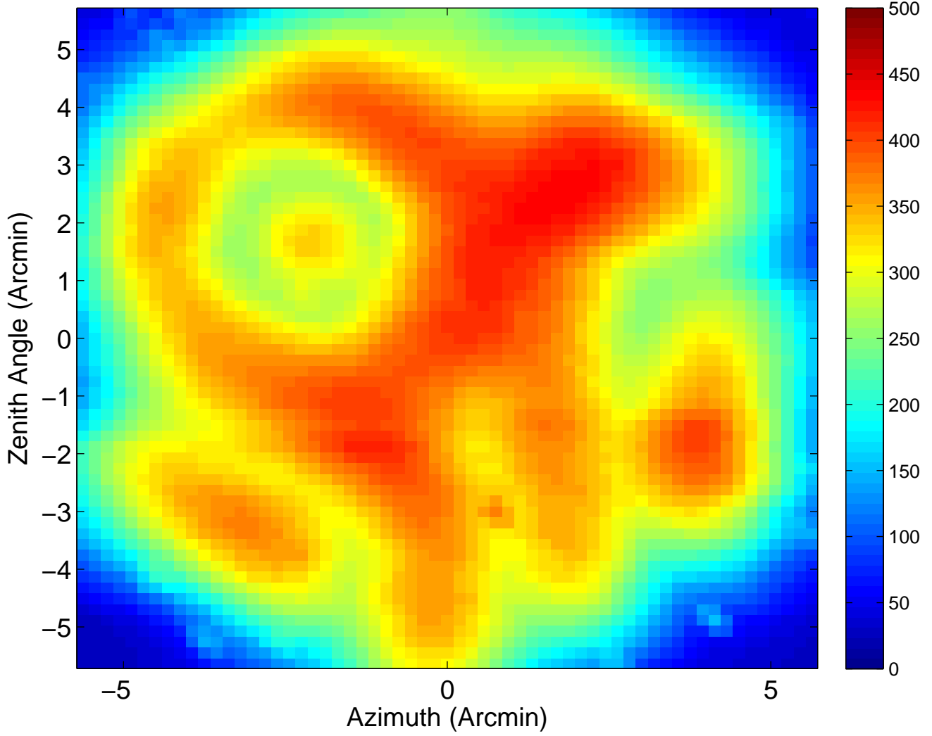
A0 Ae/Tsys Map ( z = -0.03 cm)
