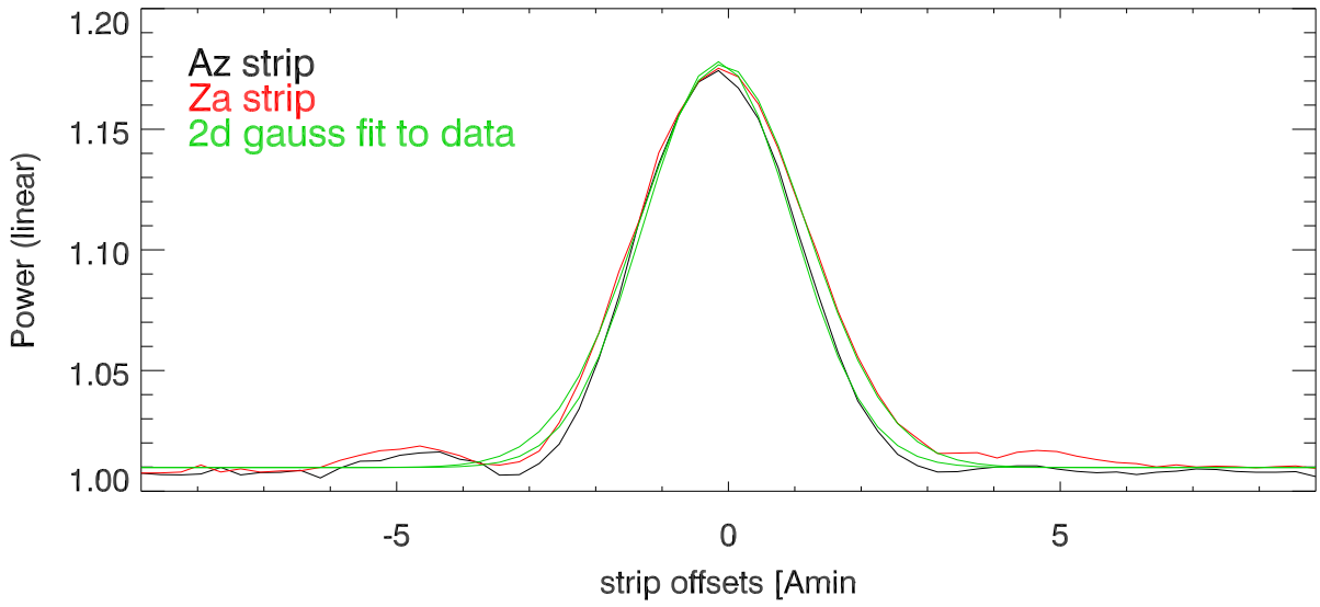
azErr: -8.6 zaErr: -4.5 Asecs... Position A0 az,za Strips
