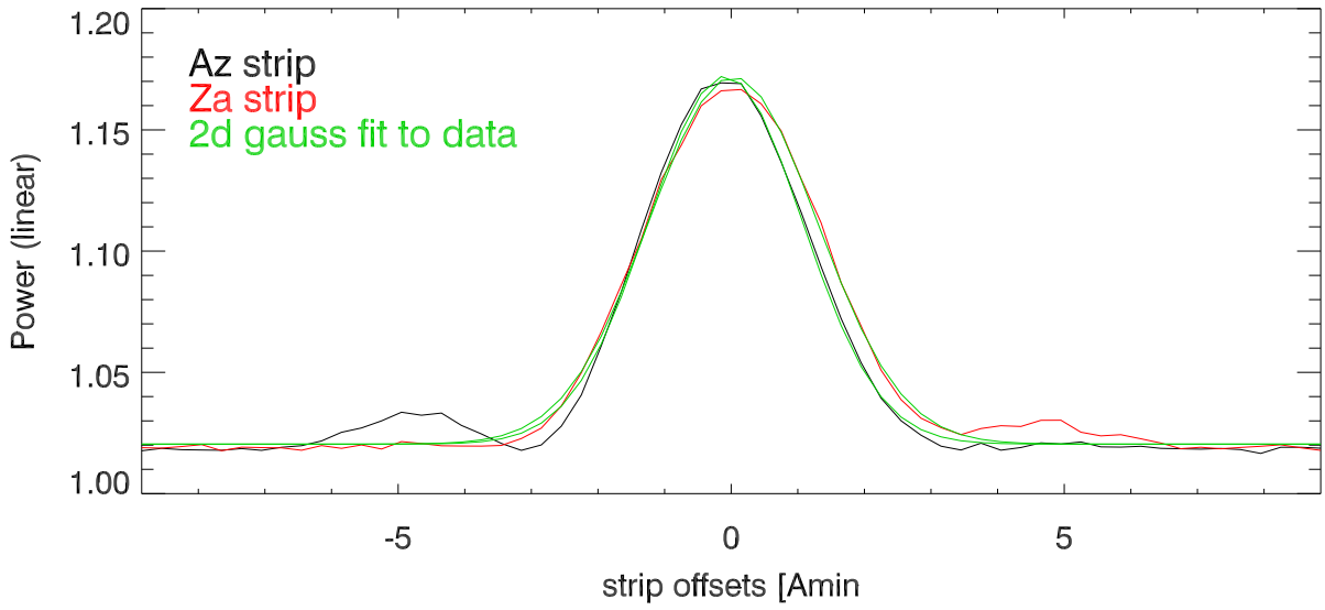
azErr: -5.3 zaErr: 1.7 Asecs... Position A3 az,za Strips
