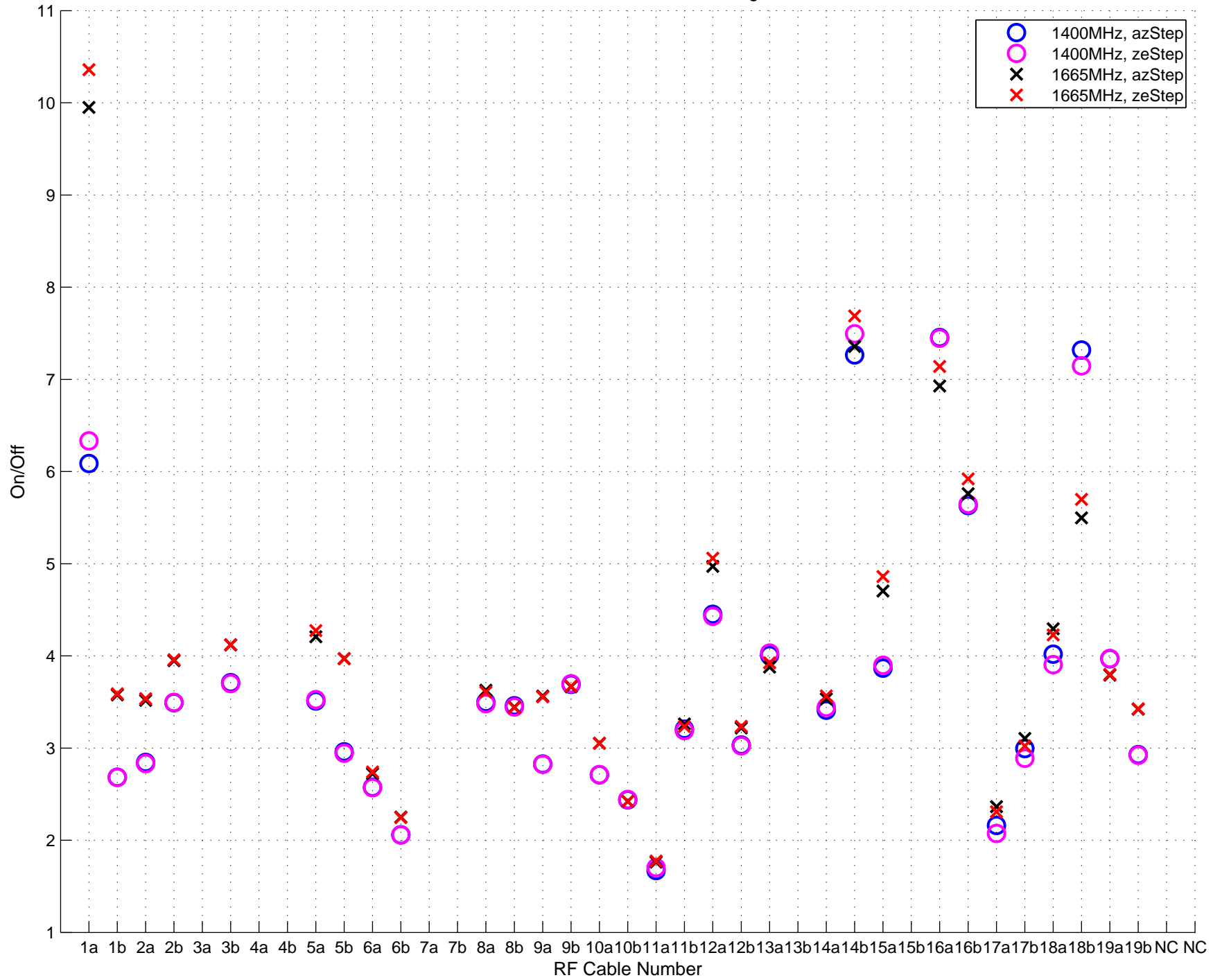
On/Off Y-Factors 1397.7539 MHz (avg across freq.) Dataset: /media/Disk0/08_03_2013_morning_moon_onoff
