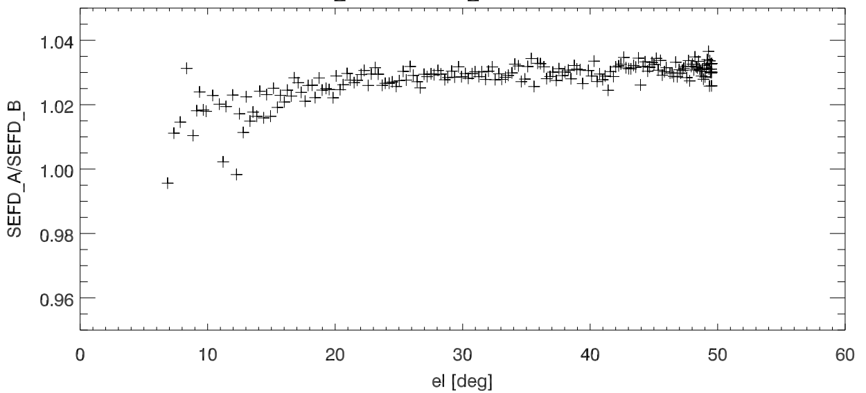
SEFD_PolA / SEFD_PolB vs elevation
