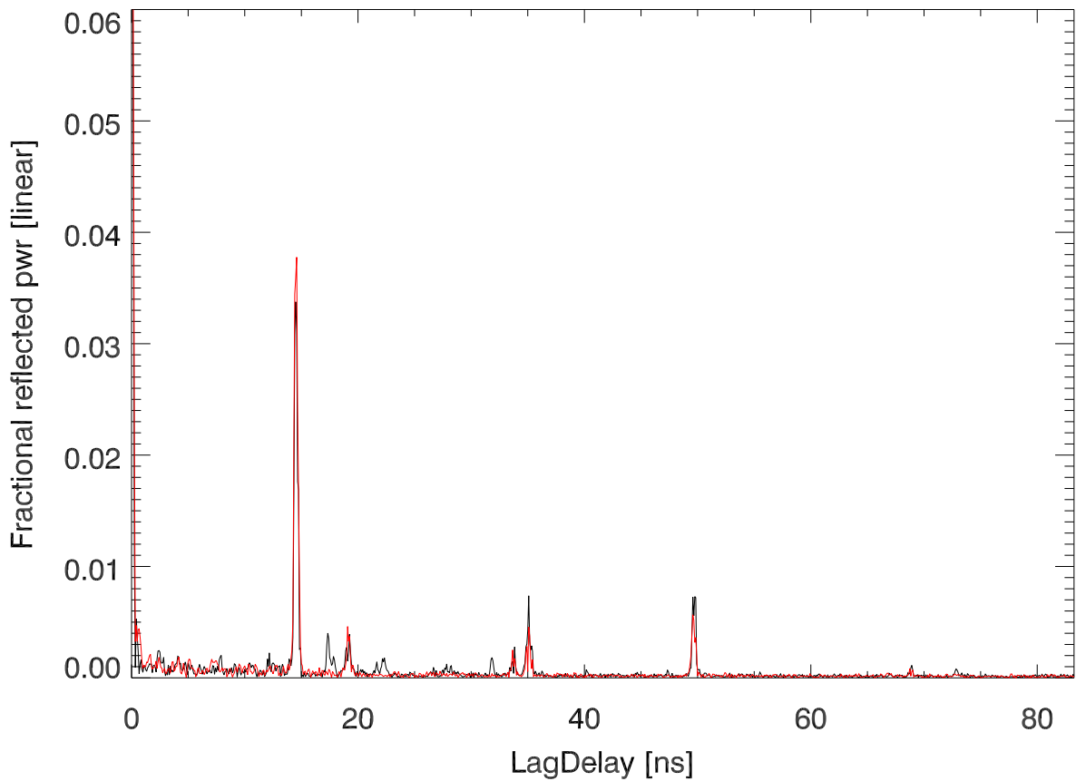
ACF of S11,S22
