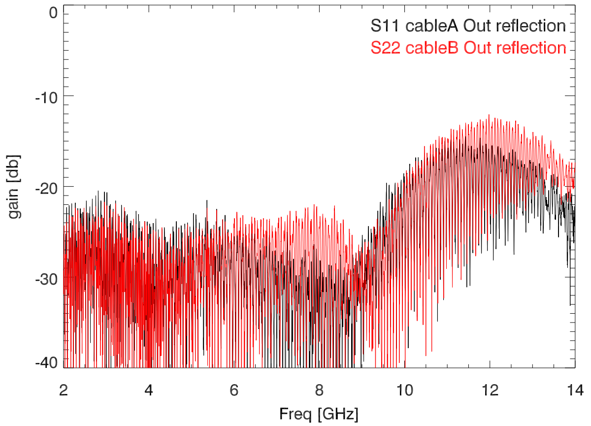
S11,S22 vs freq. (reflected from cableA,CableB)
