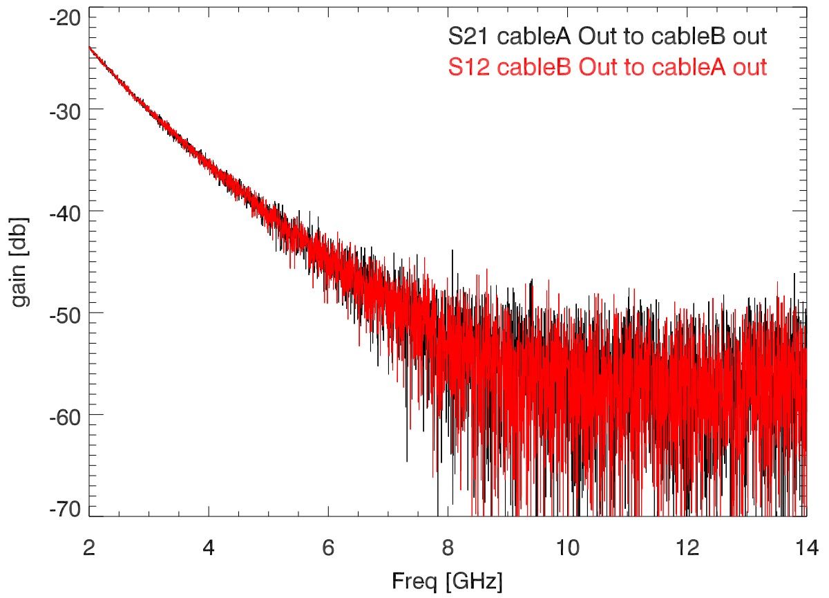
13apr23 S21 vs freq (cblA input to cblB output)
