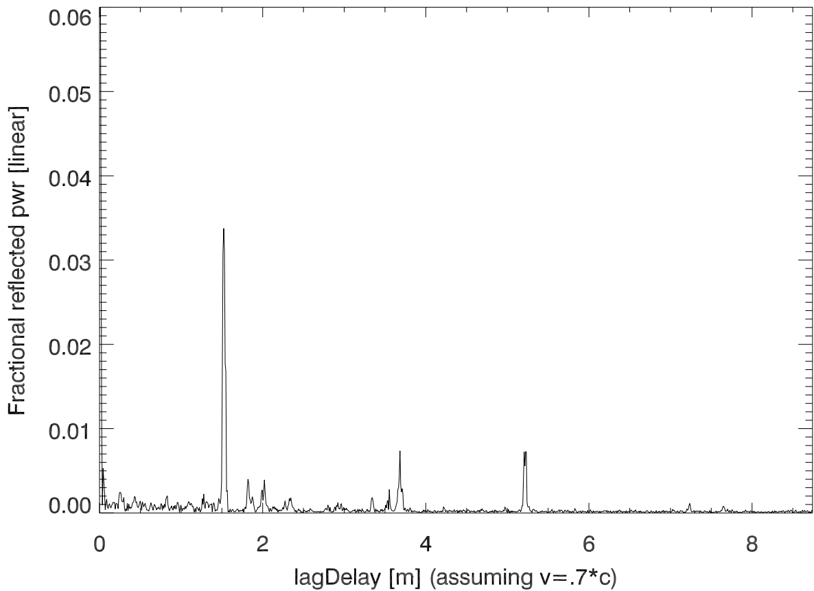
reflections single cable
