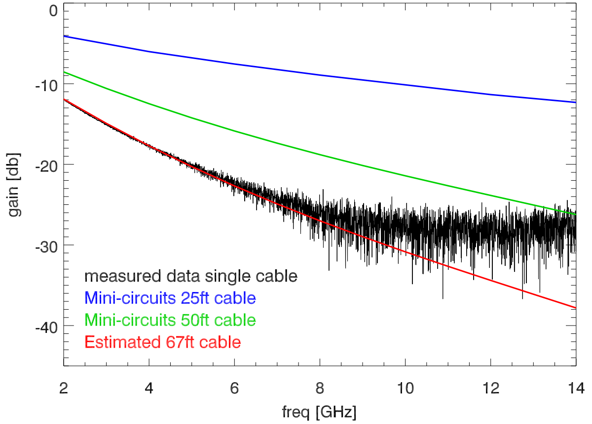
Loss single cable
