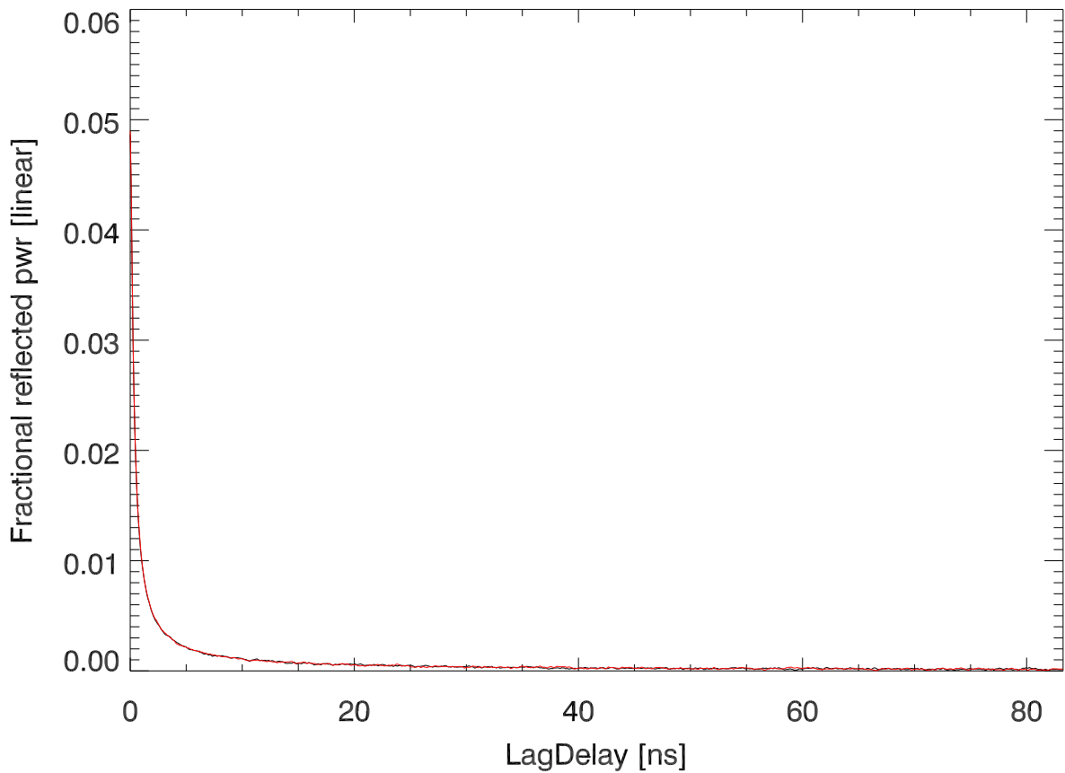
ACF of S21,S12
