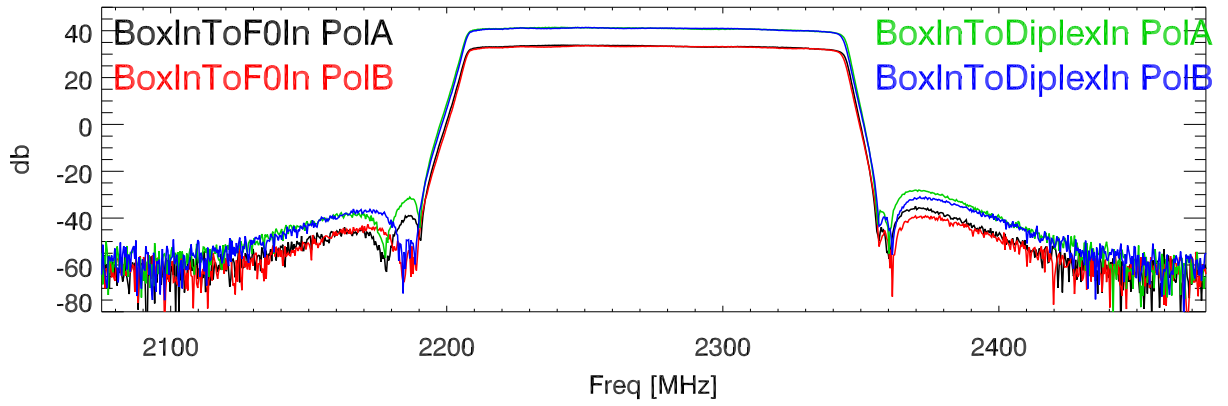
220311 S-parameters for sb postamp chassis. S21
