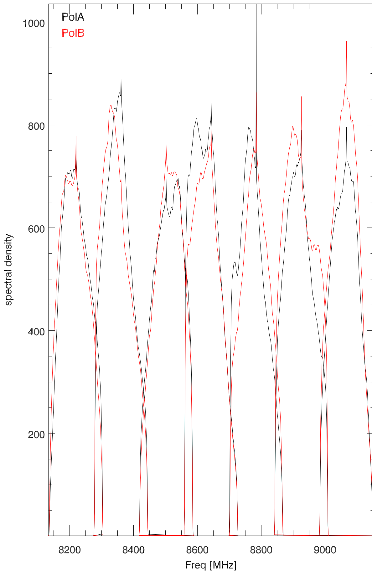
17dec21 12m xb vela psr bandpass. avg 1 rec
