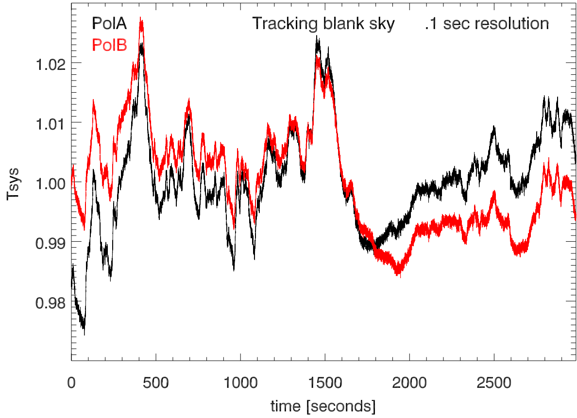
210426 12m totalPwr(172Mhz) vs time. Cfr:9116 MHz
