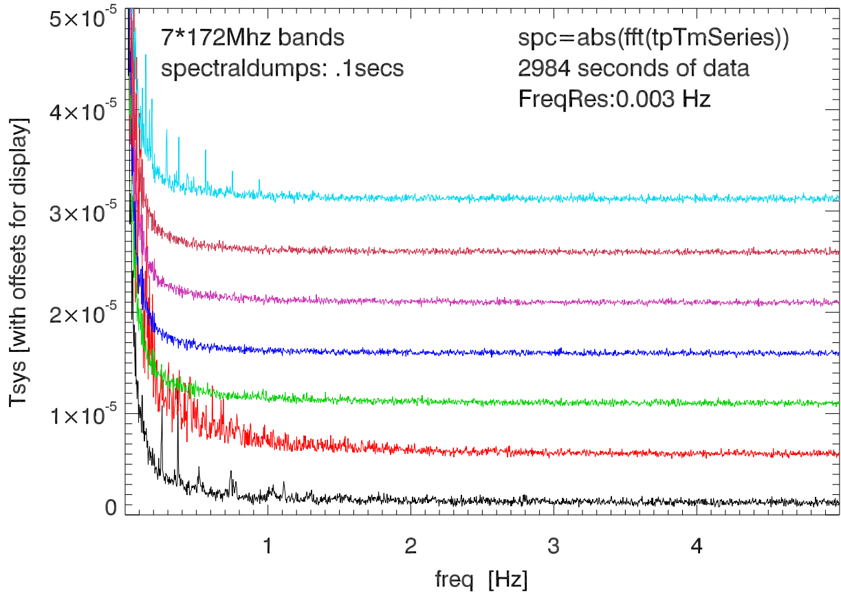
210426 12m xband spectral magnitude of total power. Pol A
