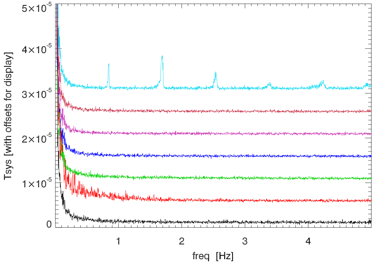
210426 12m xband spectral magnitude of total power. Pol B
