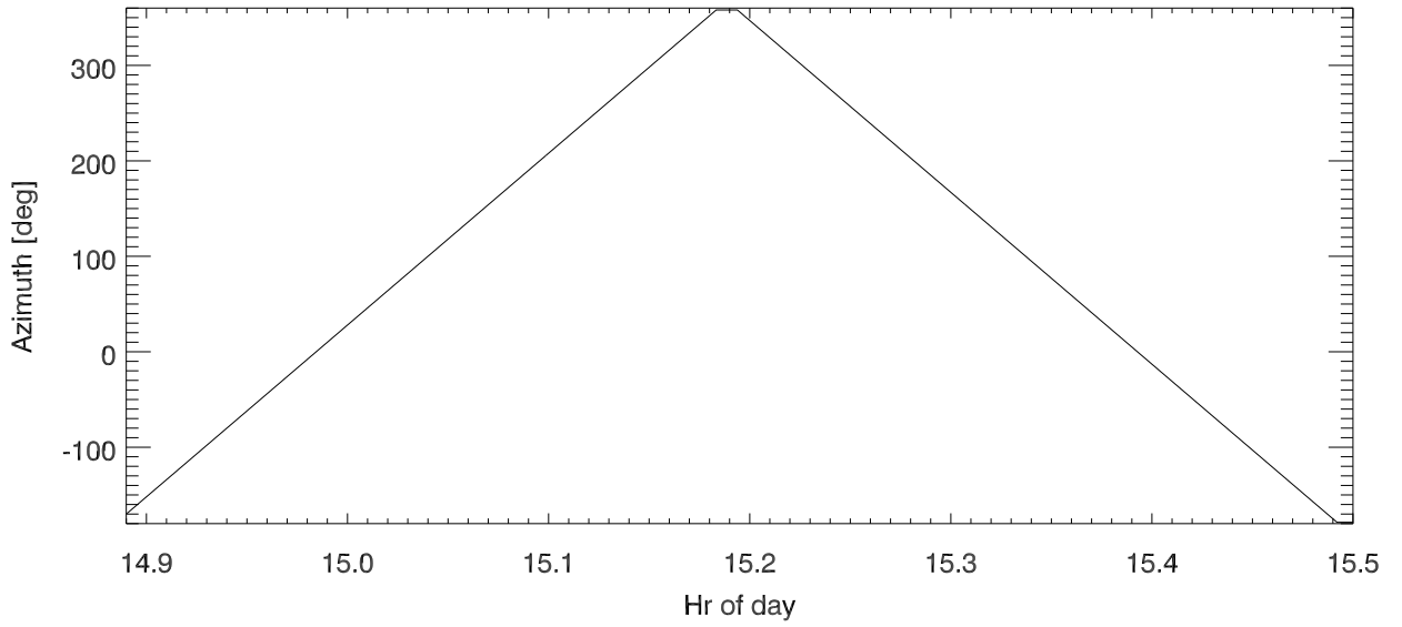
21jan22 az spin -180 to 360 @ .5deg/sec. AzPos vs time
