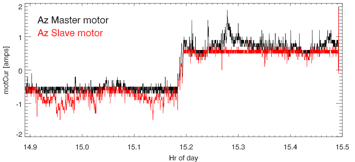
Az motor current vs time
