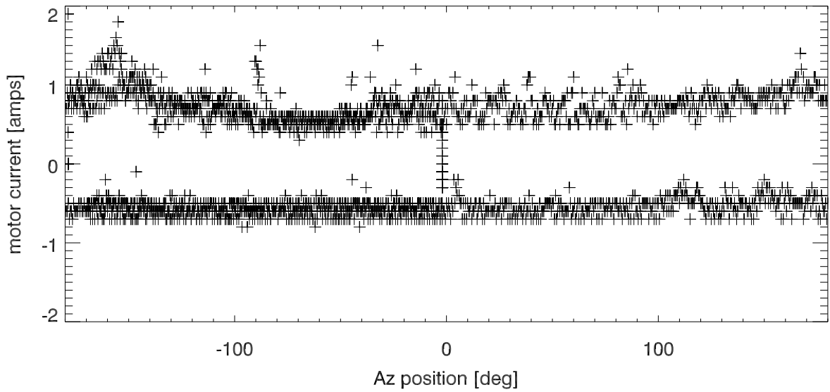
Motor Current vs az position. (Master motor)
