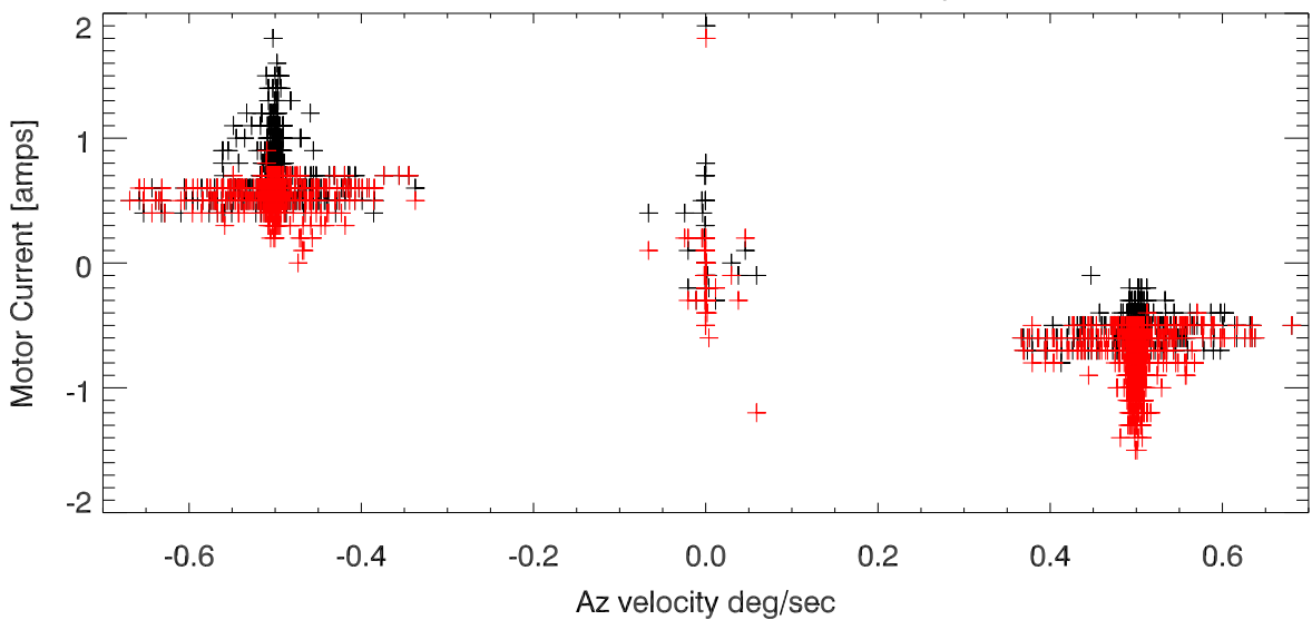
Az motor current vs azVelocity
