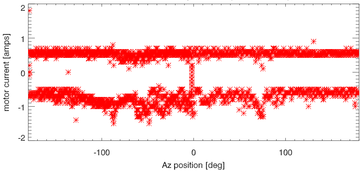
Motor Current vs az position. (Slave motor)
