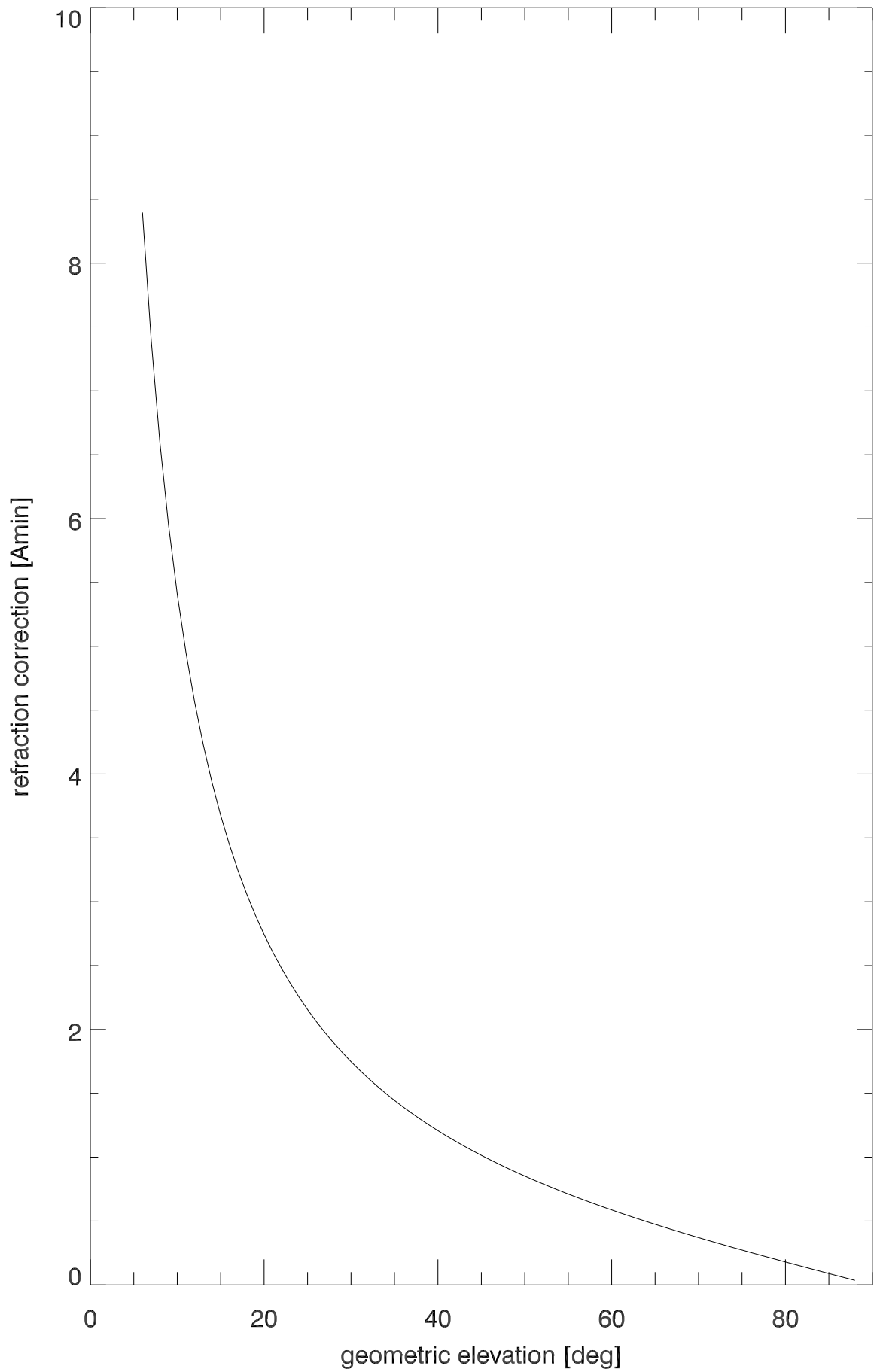
Refraction correction (Elapparent - Elgeometric) vs elevation
