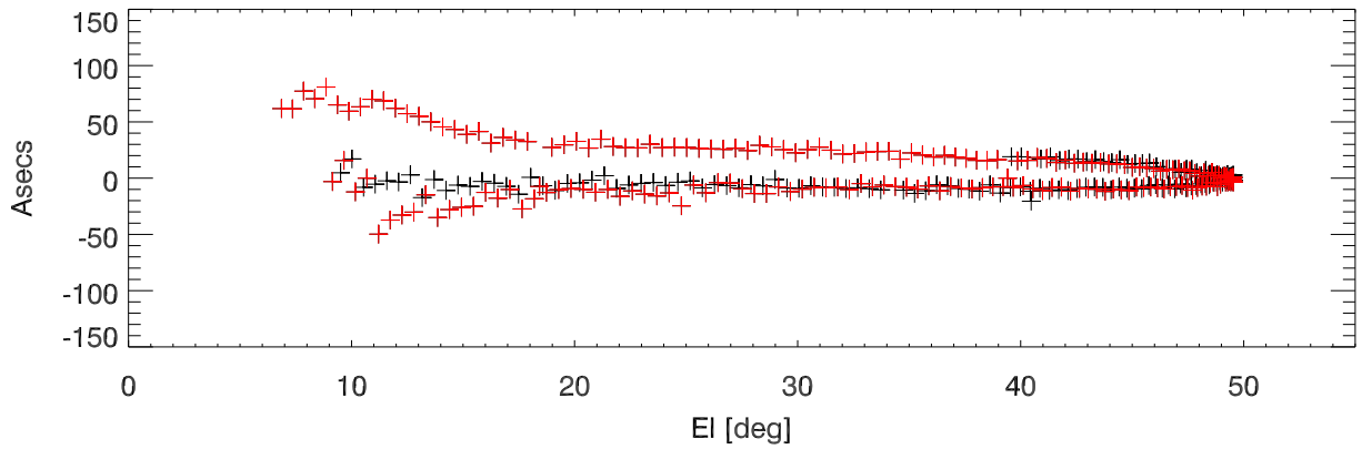
3C461 az pointing errors vs Elevation
