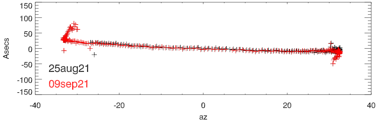
3C461 az pointing errors vs azimuth (using model3B)
