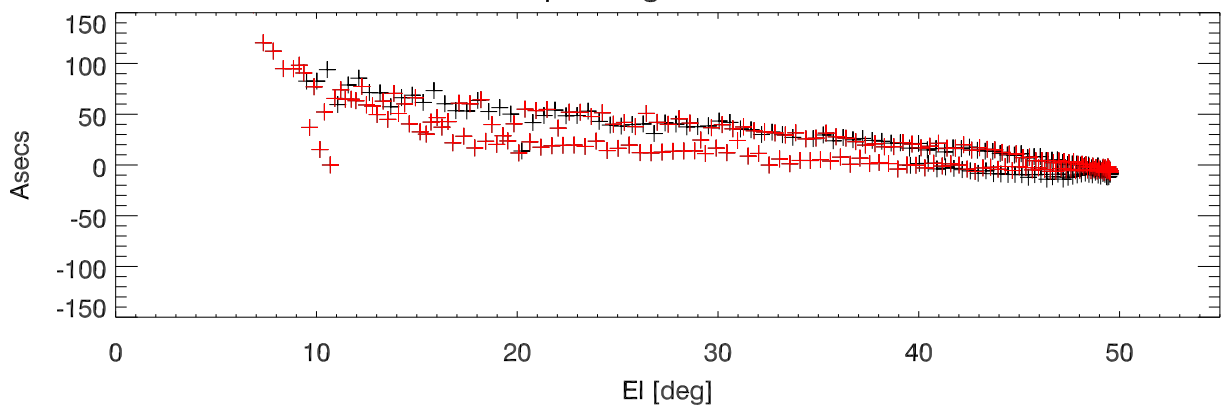
3C461 El pointing errors vs elevation
