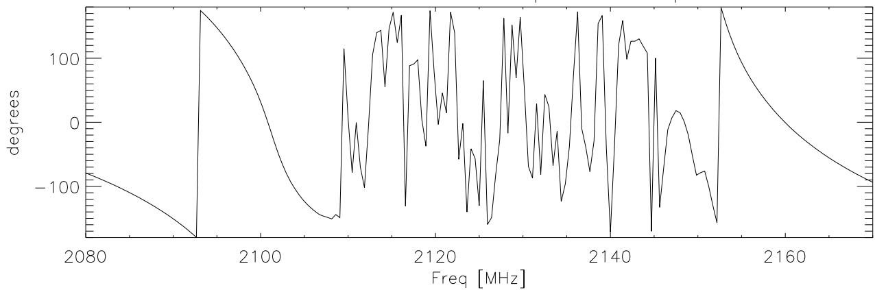
SBW notched filter S21 phase. blowup
