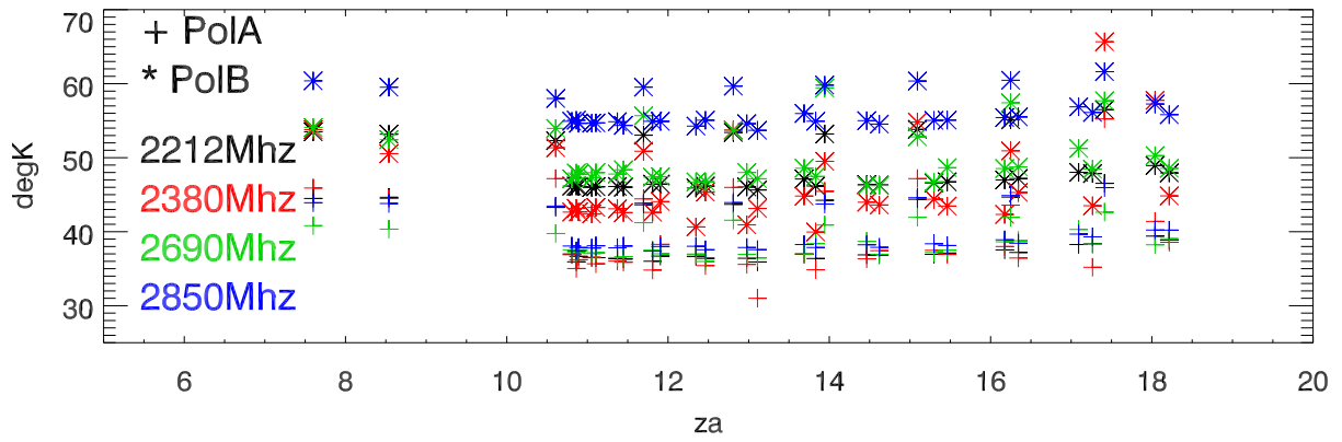
2017 sbw Calib runs. PoIA,PoIB Tsys Vs Za
