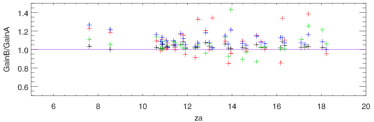
GainPoIB/GainPoIA Vs Za
