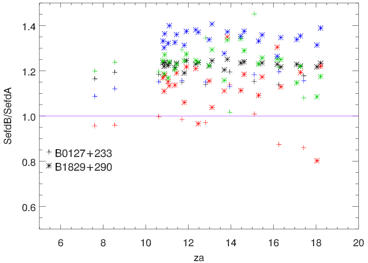
SEFDPoIB/SEFDPoIA Vs Za
