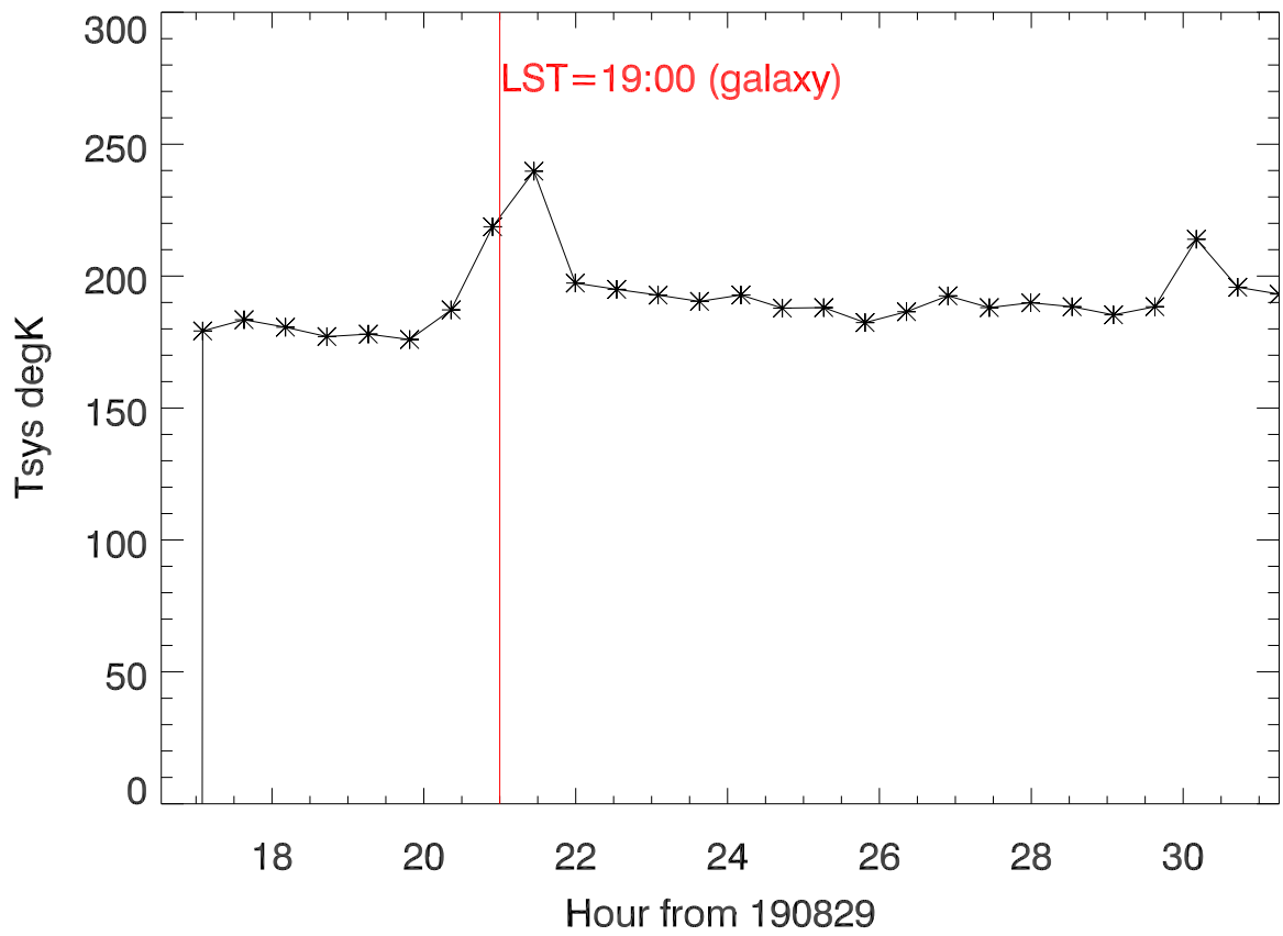
190829 Tsys vs Hour of day.(430rcv warmup at 20:00)
