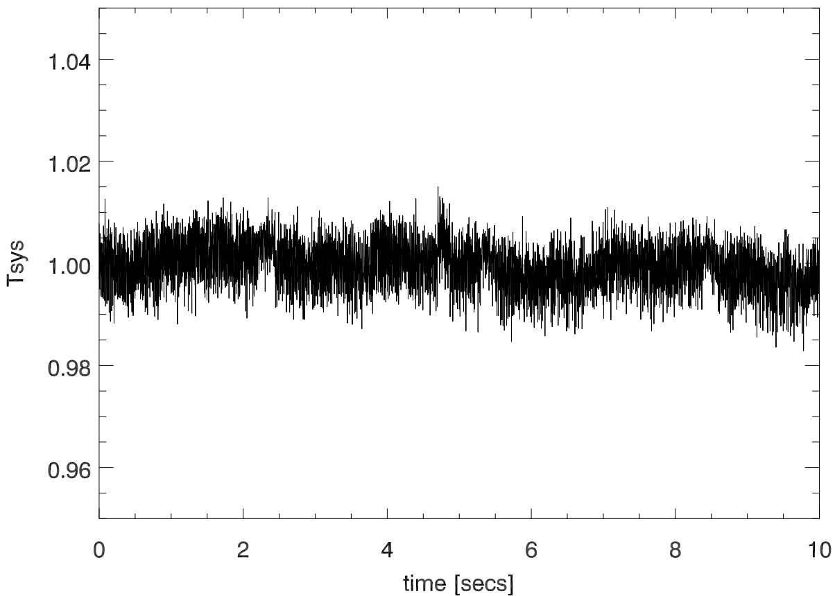
20feb14 p1693 file.0300 total power vs time
