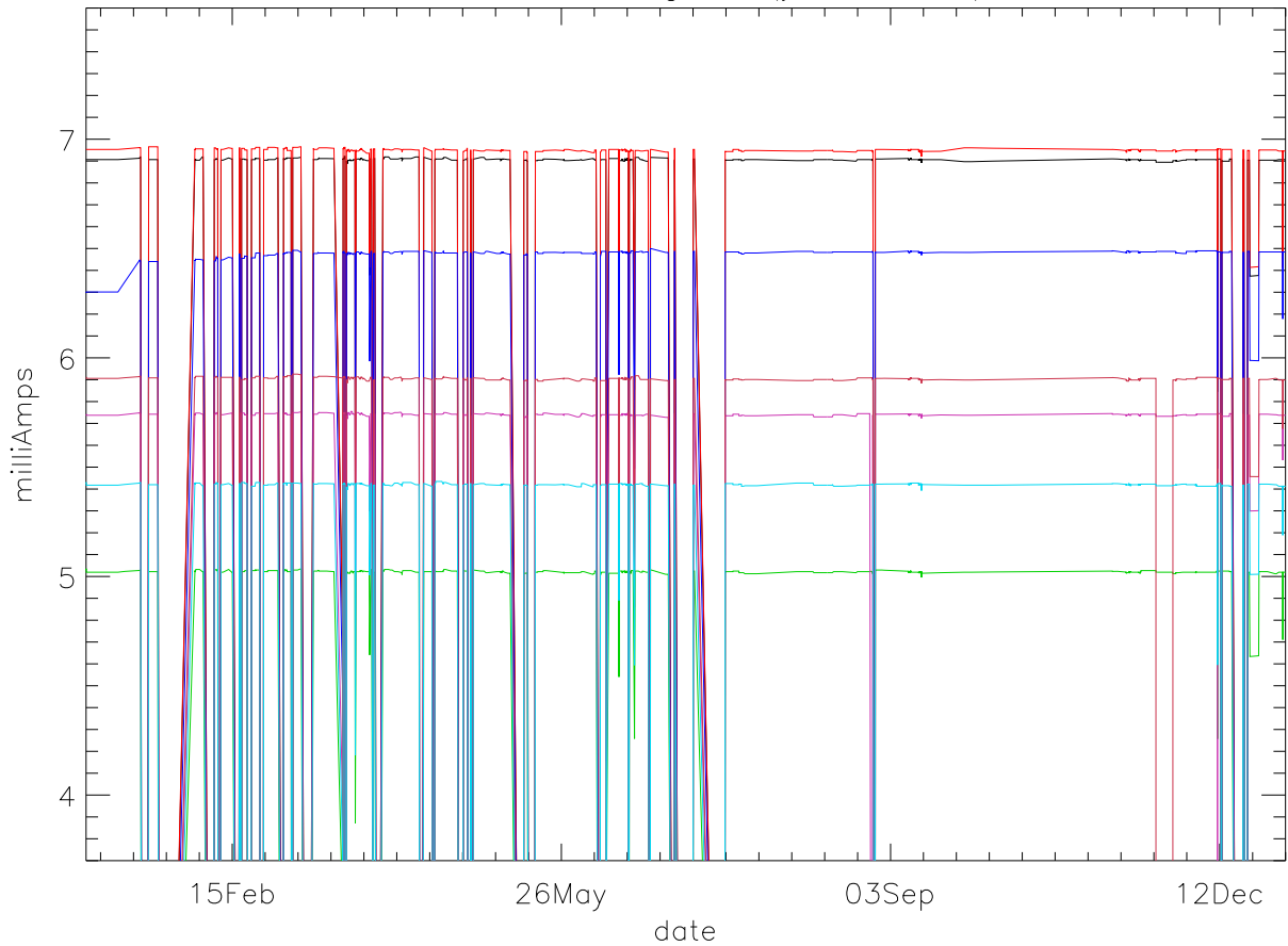
Id:Drain Current. stage 1 (year 2017) PoIB
