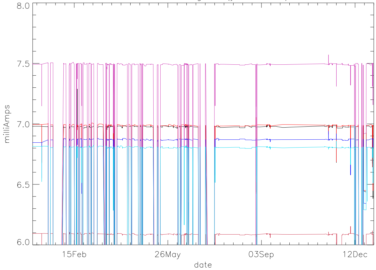
Id:Drain Current. stage 3 (year 2017) PoIB
