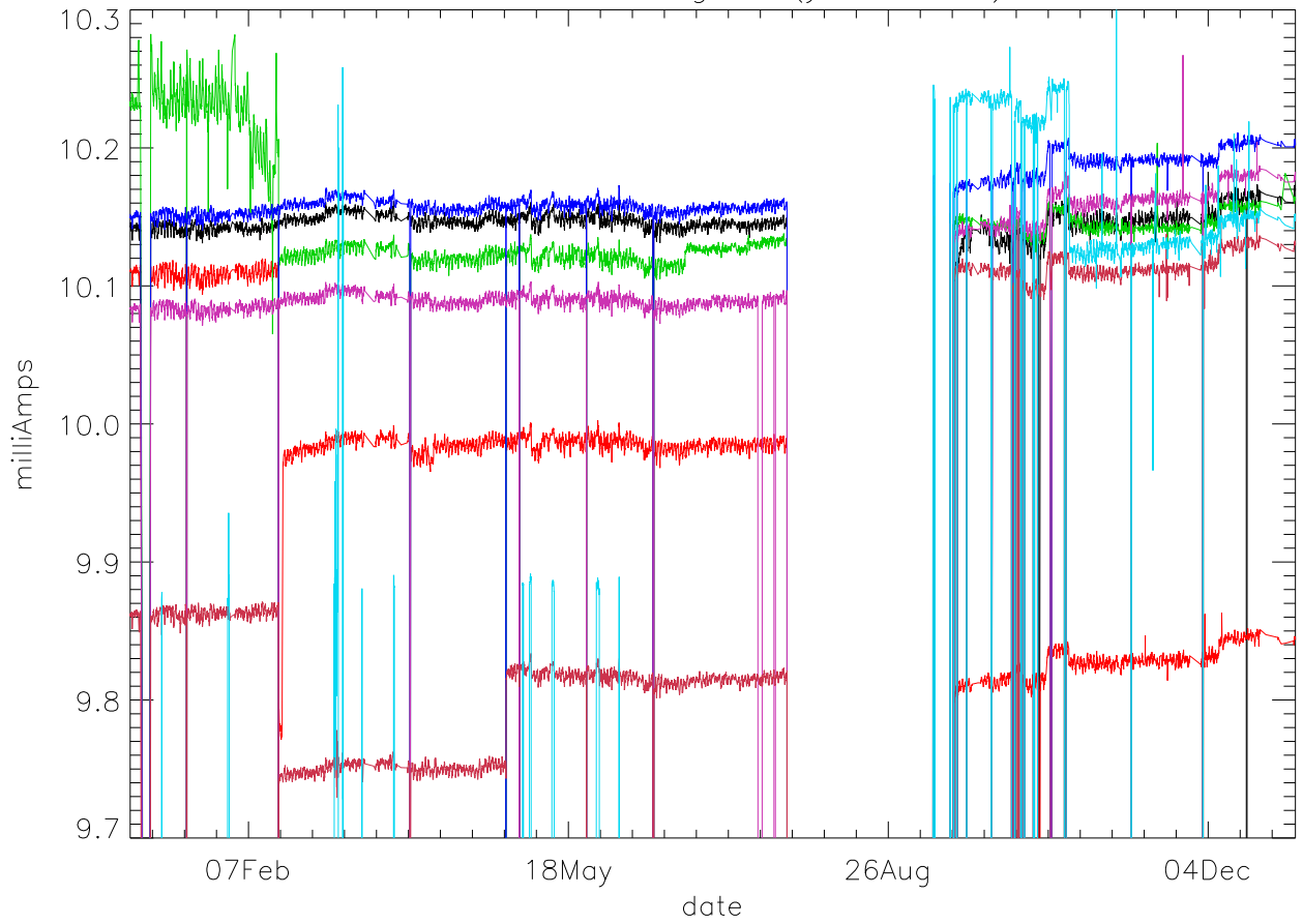
Id:Drain Current. stage 2 (year 2011) PoIB
