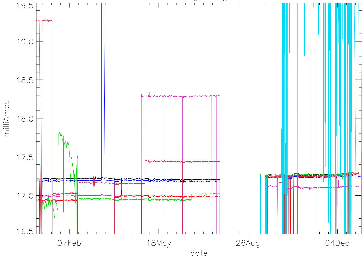
Id:Drain Current. stage 3 (year 2011) PoIB
