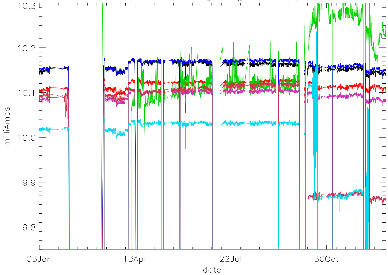
Id:Drain Current. stage 2 (year 2010) PoIB
