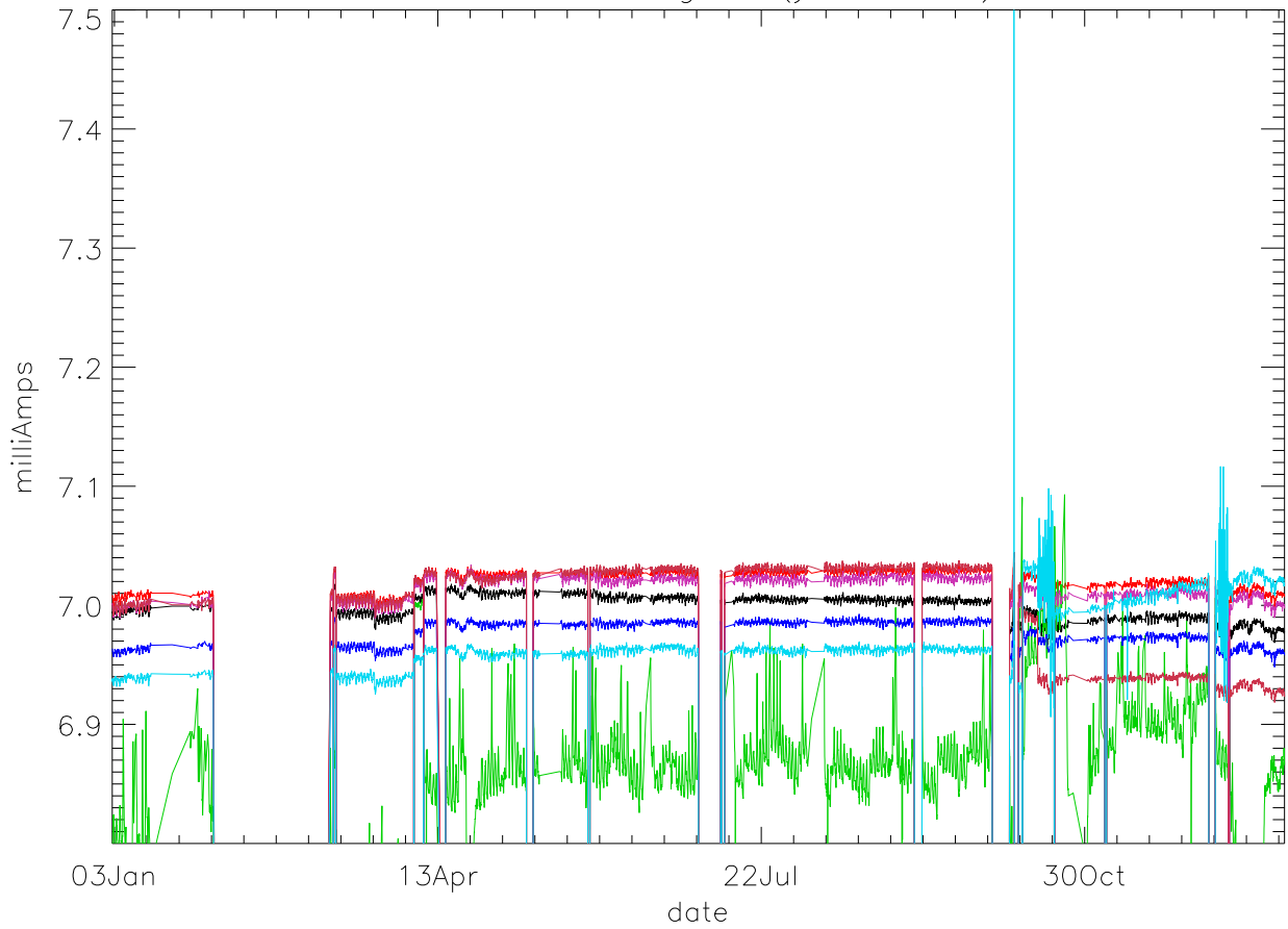
Id:Drain Current. stage 1 (year 2010) PoIB
