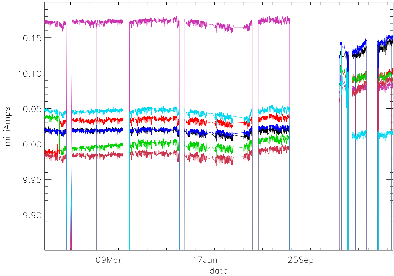
Id:Drain Current. stage 2 (year 2009) PoIB
