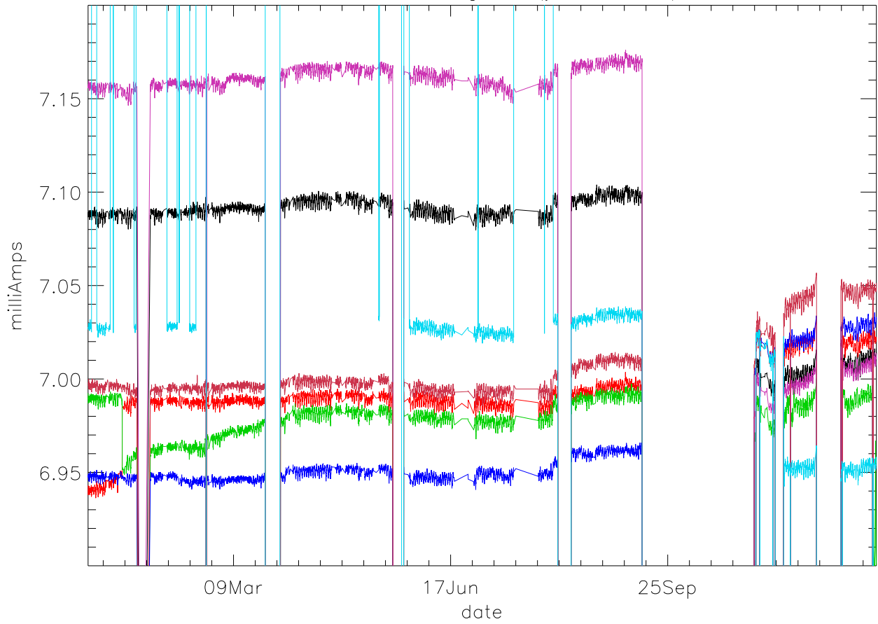
Id:Drain Current. stage 1 (year 2009) PoIB
