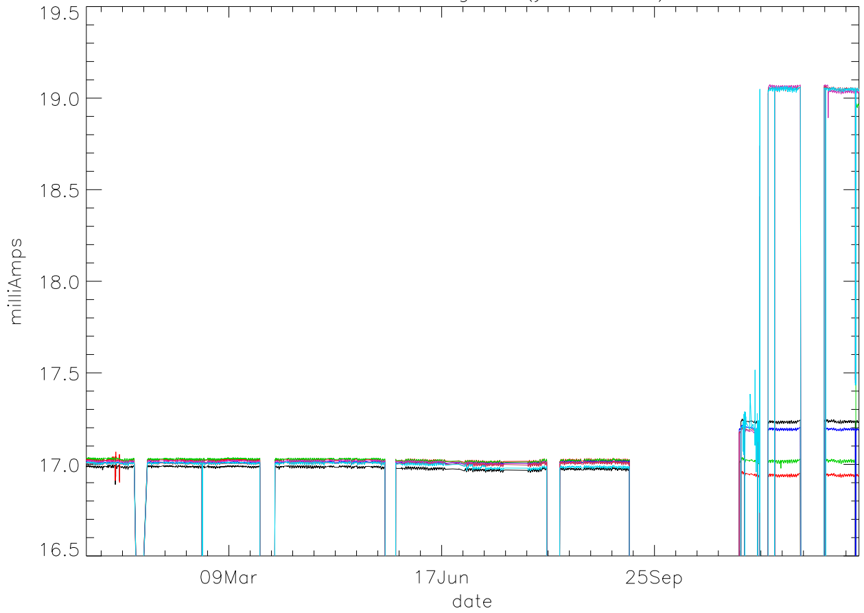
Id:Drain Current. stage 3 (year 2009) PoIB
