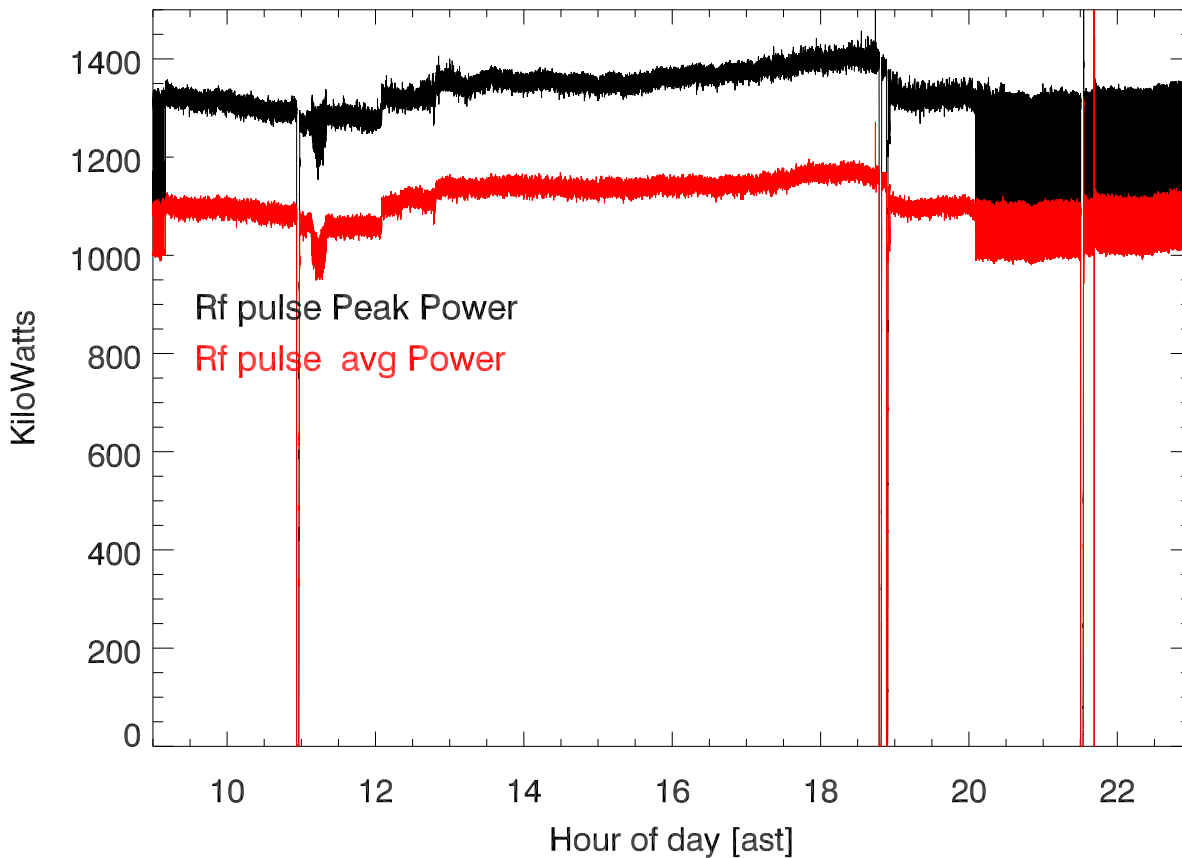
20180318 X115 430tx power (dome) vs hour of day
