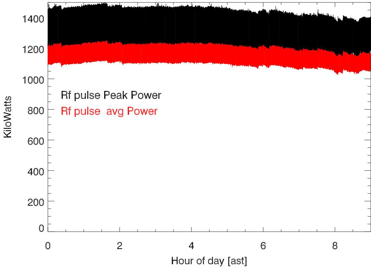
20180320 T3239 430tx power (dome) vs hour of day
