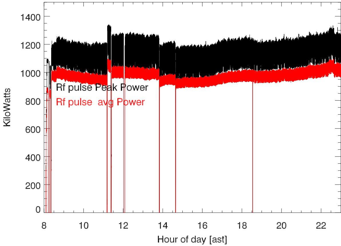
20180215 T1193 430tx power (dome) vs hour of day
