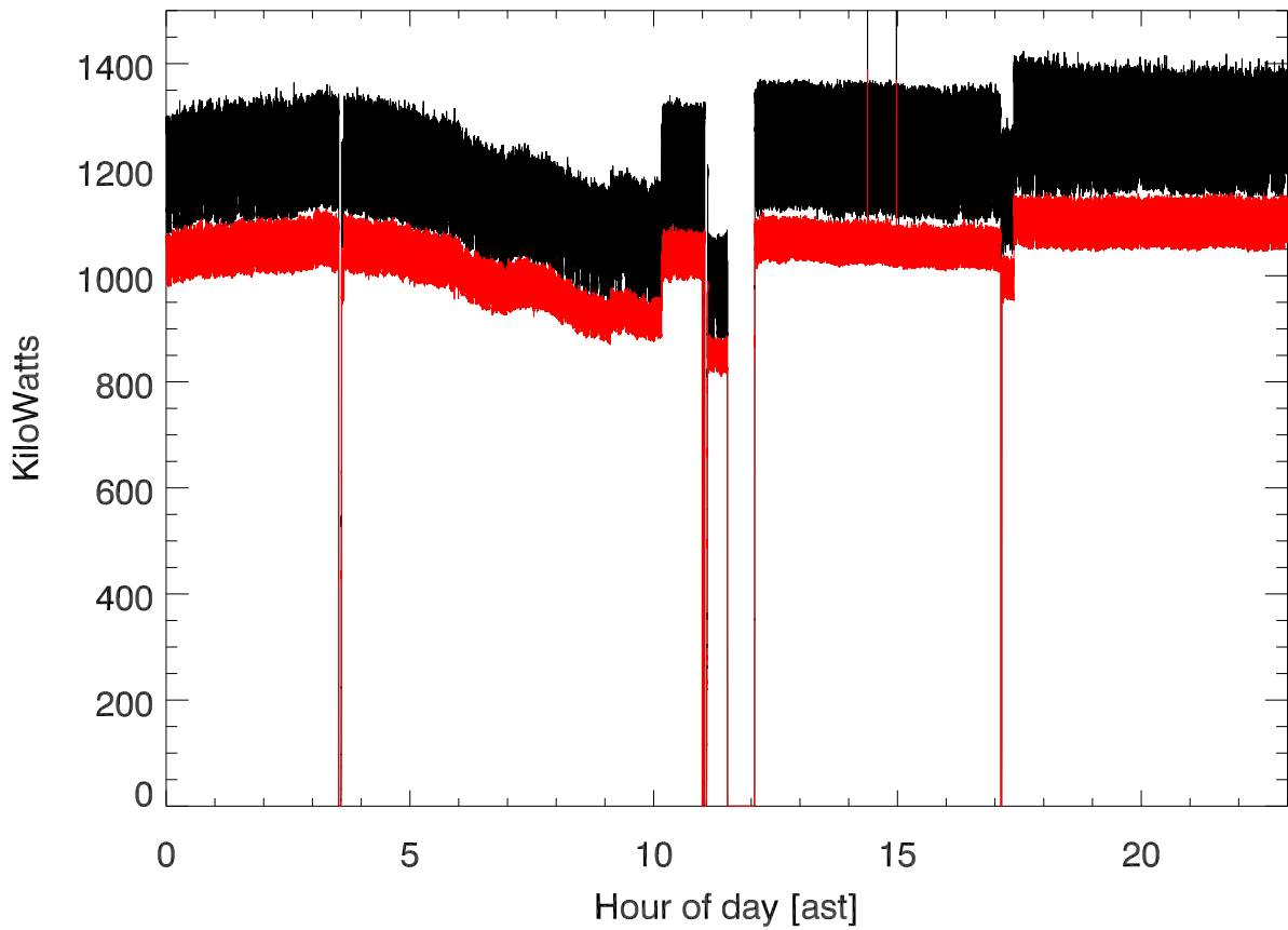
20180216 T1193 430tx power (dome) vs hour of day
