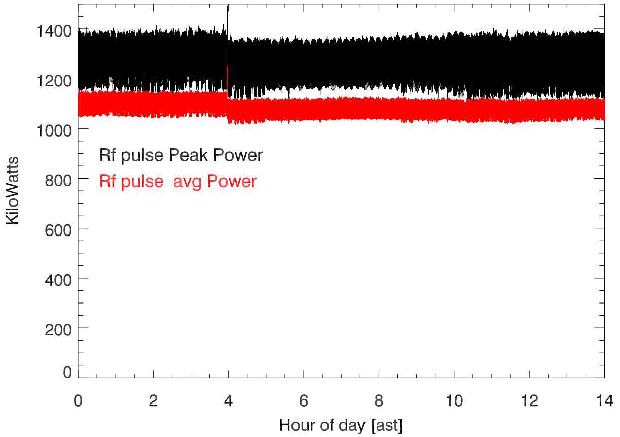
20180217 T1193 430tx power (dome) vs hour of day
