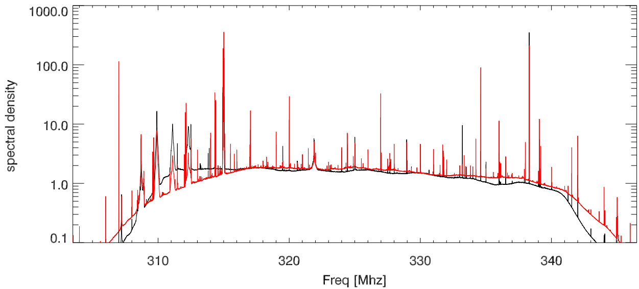
max hold Spectra from 10 cross patterns
