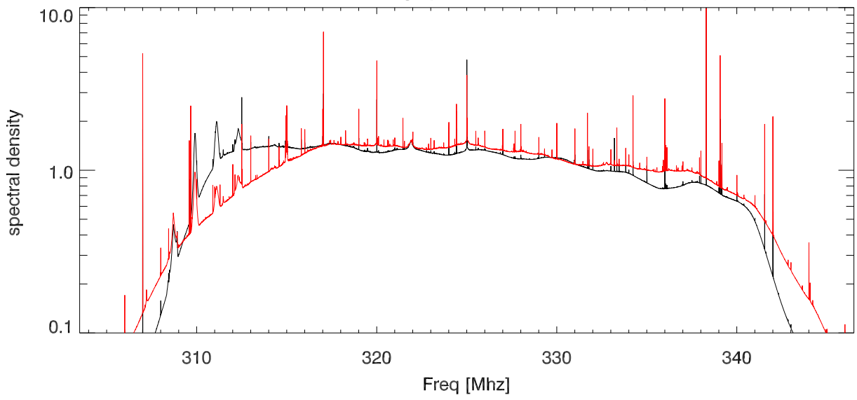
median Spectra from 10 cross patterns
