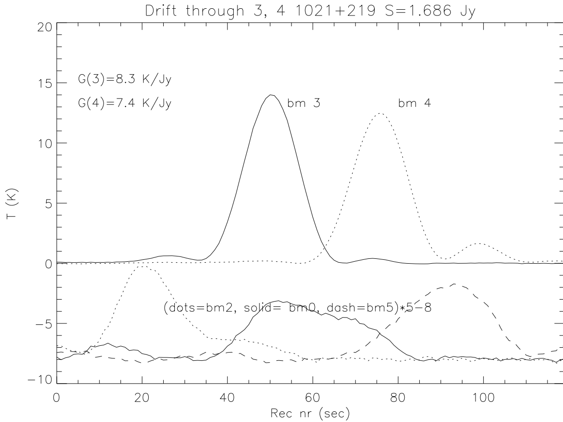
Fig. 3.— Drift 3: continuum power with source 1021+219 going through beams 3 and 4. Tracings for the center group (beams 2, 0 and 5) were blown up by a factor 5 and offset for overplotting.
