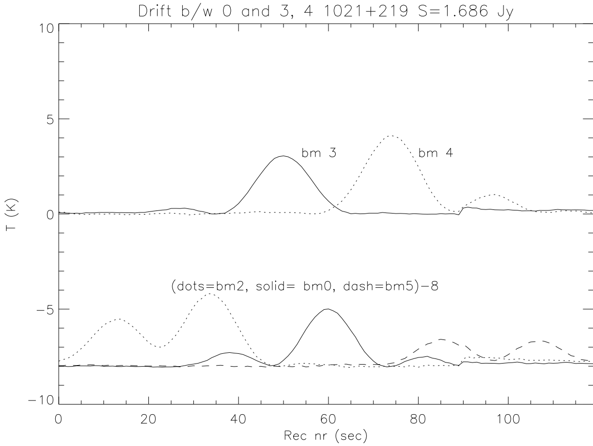
Fig. 5.— Drift 5: continuum power with source 1021+219 going between beam group (2, 0, 5) and group (3, 4). Tracings for the center group (beams 2, 0 and 5) were offset for overplotting. In this drift the source runs 2' 30" from the nominal center group of beams, and 2' 30" from the outer one.
