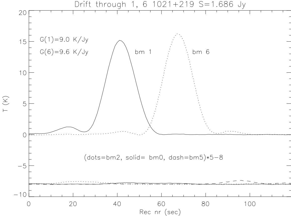
Fig. 2.— Drift 2: continuum power with source 1021+219 going through beams 1 and 6. Tracings for the center group (beams 2, 0 and 5) were blown up by a factor 5 and offset for overplotting.
