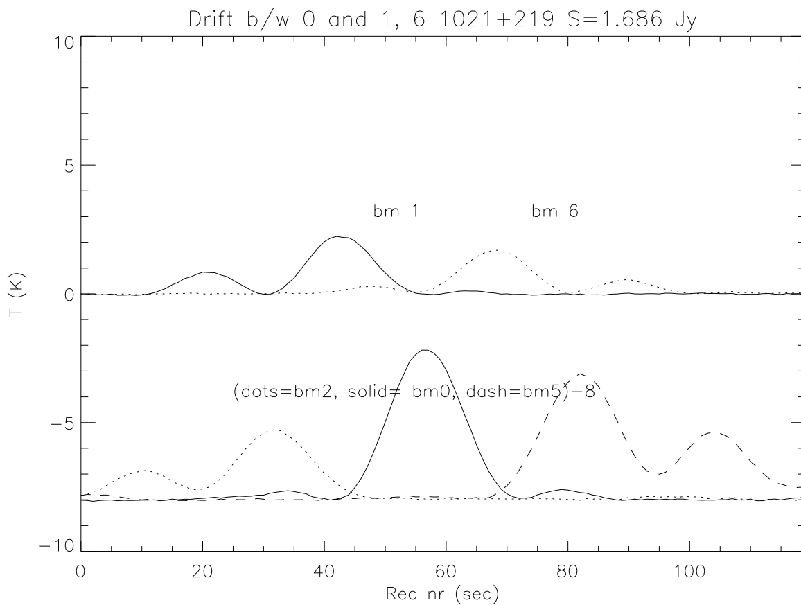
Fig. 4.— Drift 4: continuum power with source 1021+219 going between beam group (2, 0, 5) and group (1, 6). Tracings for the center group (beams 2, 0 and 5) were offset for overplotting. In this drift the source runs only 2' 10'' from the nominal center group of beams, and 2' 50'' from the outer one.
