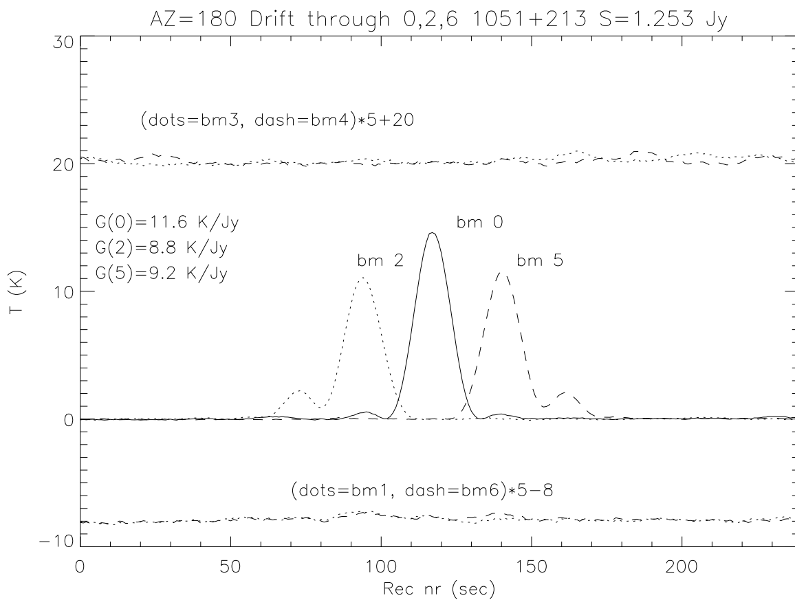
Fig. 6.— Drift 6: continuum power with source 1051+213 nominally going through the centers of beam group (2, 0, 5) and group, at AZ=180°. Tracings for the outer groups of beams were offset for overplotting.
