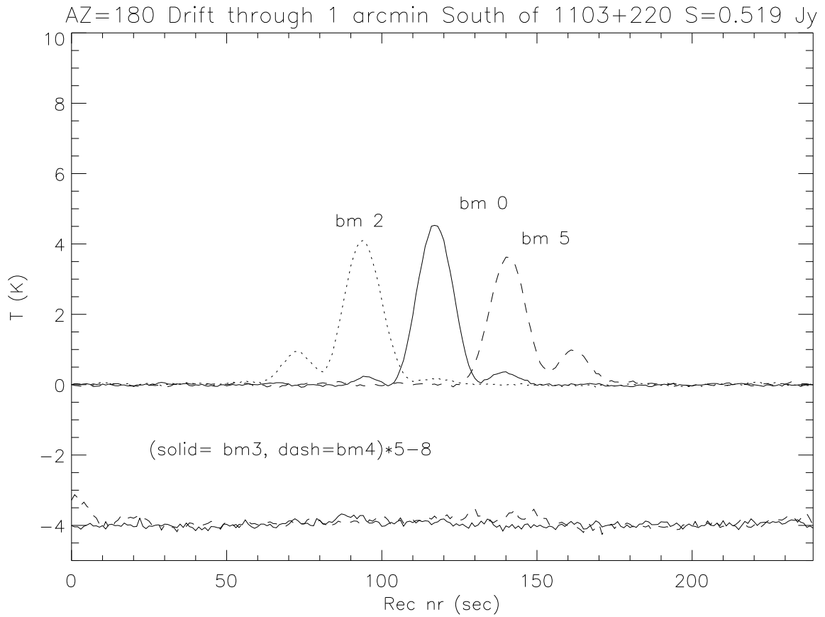
Fig. 7.— Drift 7: continuum power with source 1103+220 going between beam group (2, 0, 5) and group (3, 4) at AZ=180°. In this drift the source runs 1' from the nominal center group of beams.
