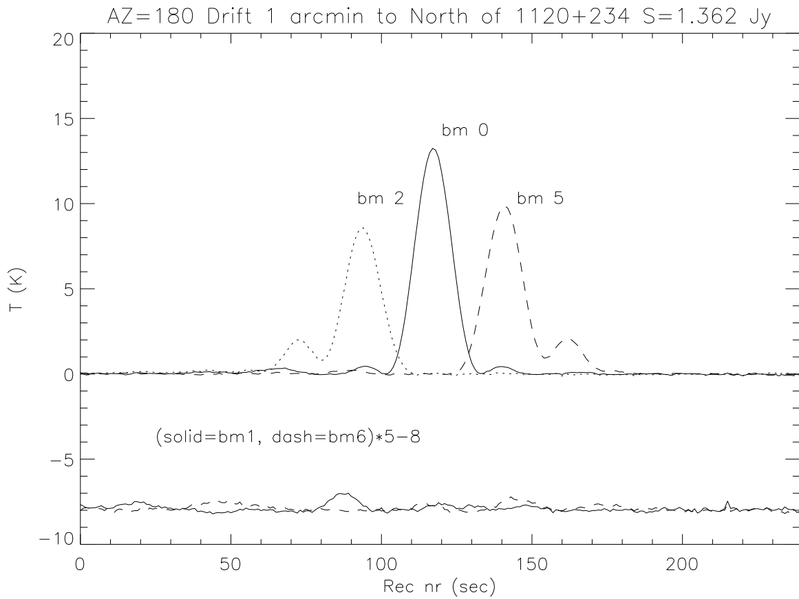
Fig. 8.— Drift 8: continuum power with source 1120+234 going between beam group (2, 0, 5) and group (1, 6) at AZ=180°. In this drift the source runs 1' from the nominal center group of beams.
