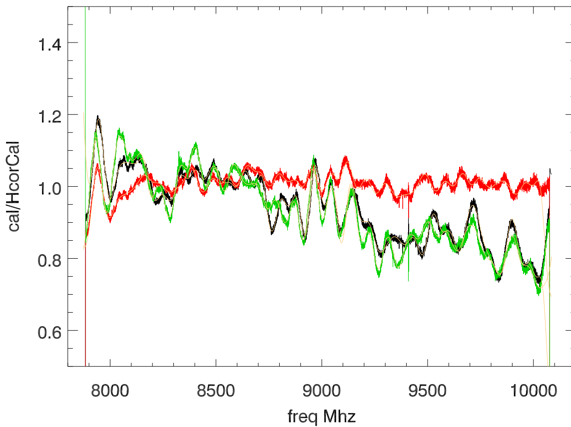
HiCals/Hcorcal polB.
