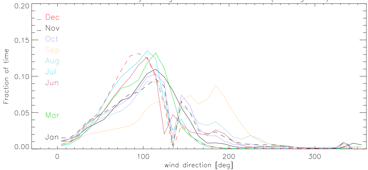
2008 Monthly histogram of wind direction (10 deg bins)
