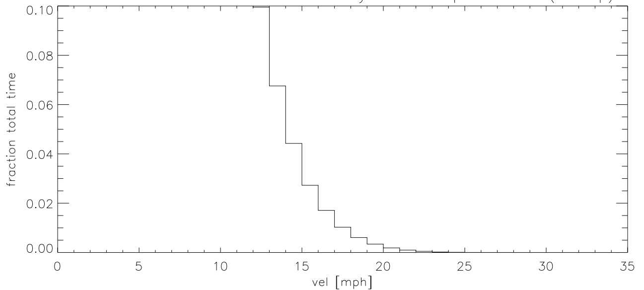
FEB20 Fraction of time wind velocity exceeds specified vel (blowup)
