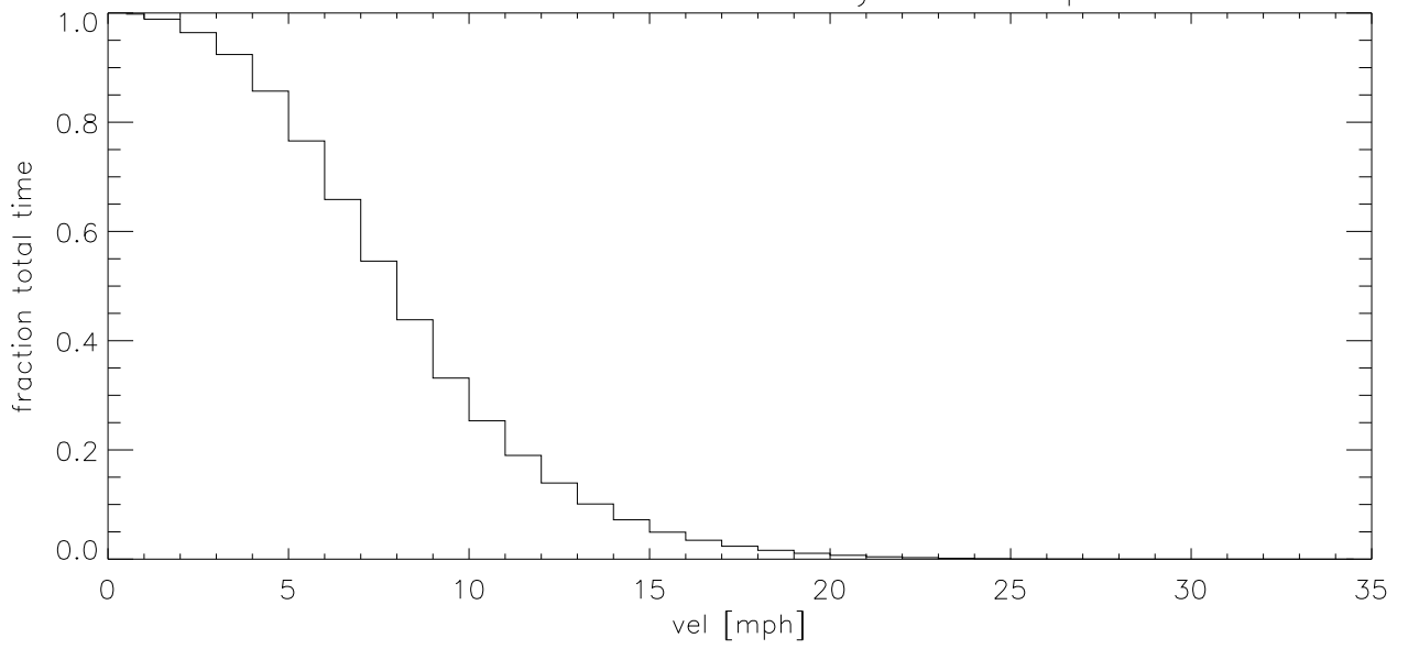
JAN20 Fraction of time wind velocity exceeds specified vel (blowup)
