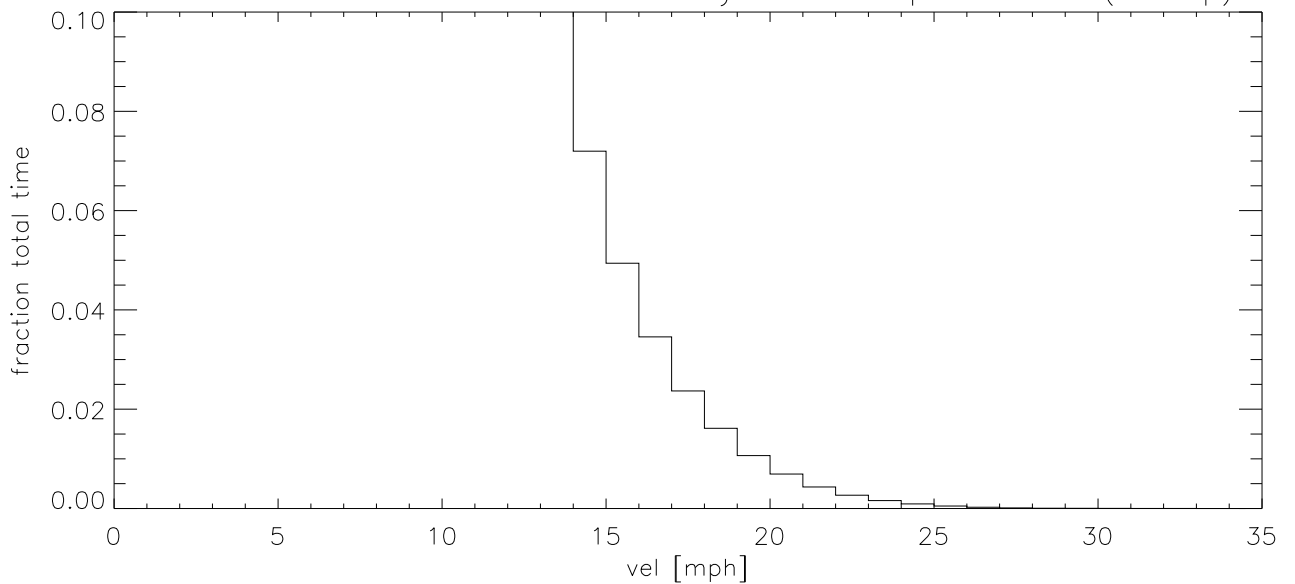
JAN20 Fraction of time wind velocity exceeds specified vel (blowup)
