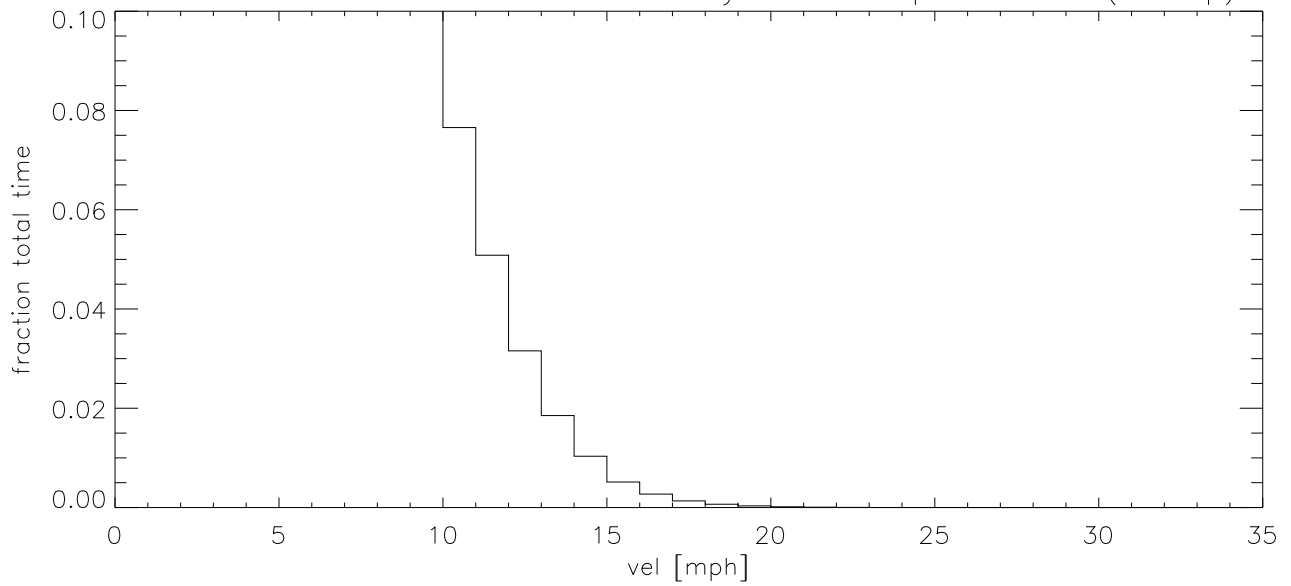
MAY19 Fraction of time wind velocity exceeds specified vel (blowup)
