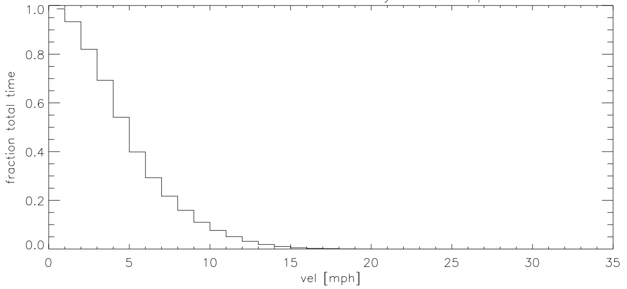
MAY19 Fraction of time wind velocity exceeds specified vel (blowup)
