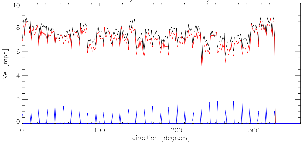
MAR19 Average, median velocity by direction
