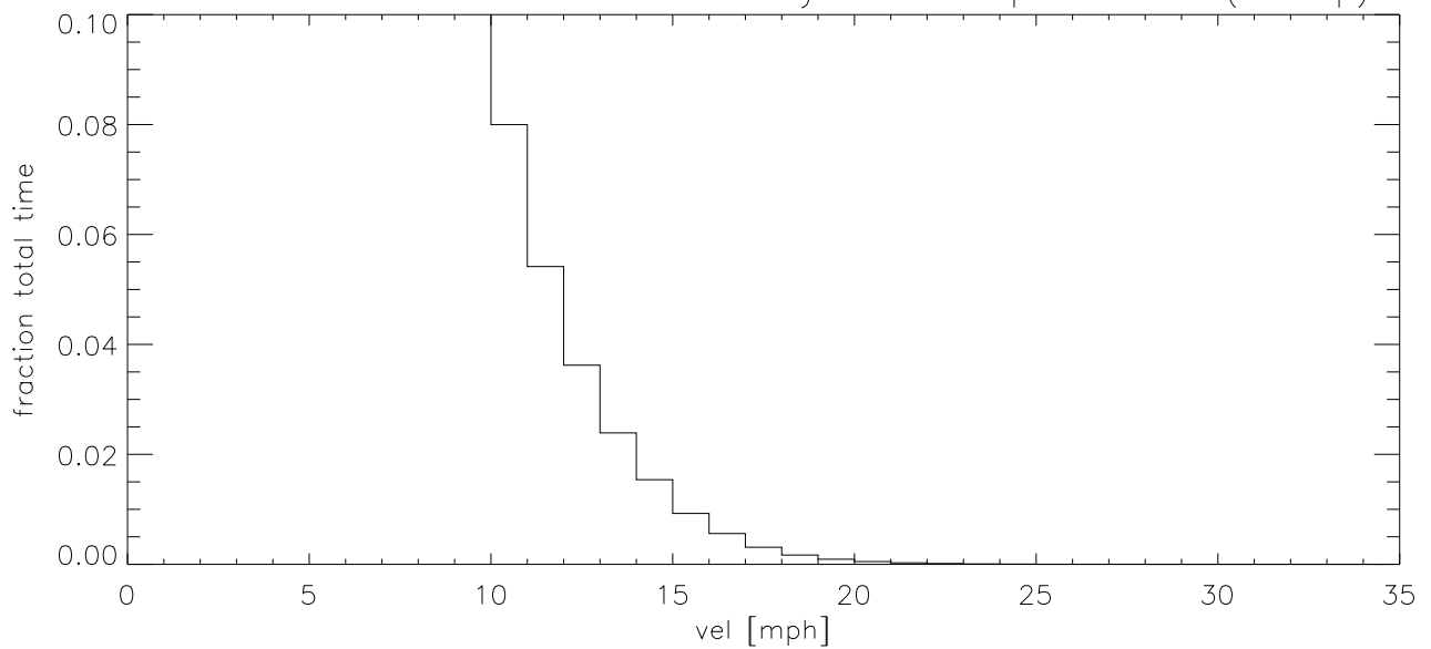
OCT18 Fraction of time wind velocity exceeds specified vel (blowup)
