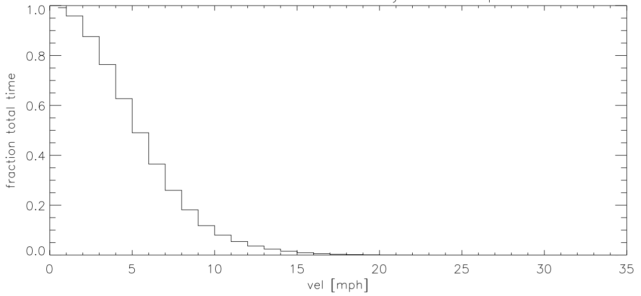
OCT18 Fraction of time wind velocity exceeds specified vel (blowup)
