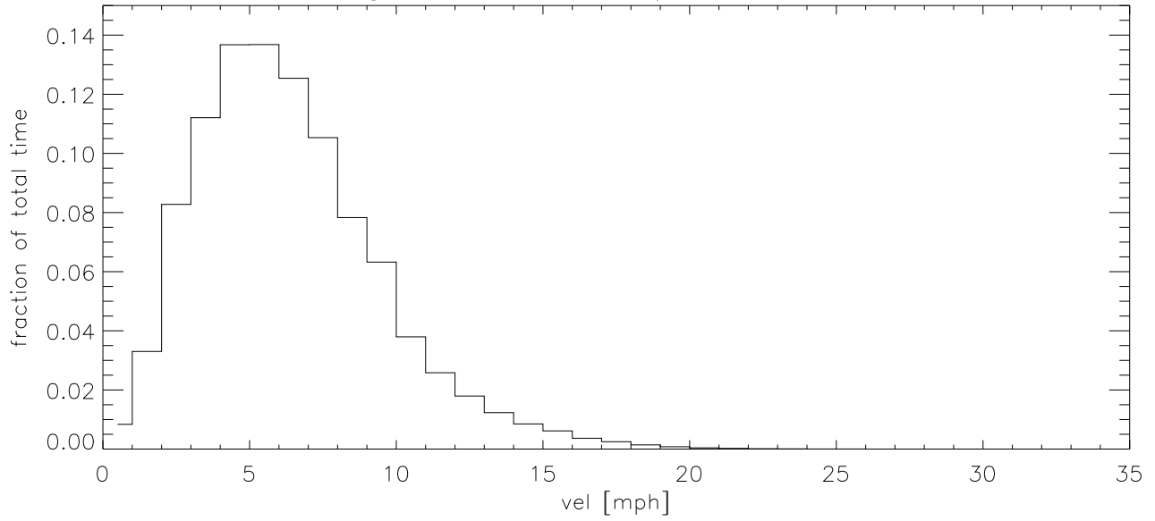
OCT18 Fraction of time wind velocity exceeds specified vel
