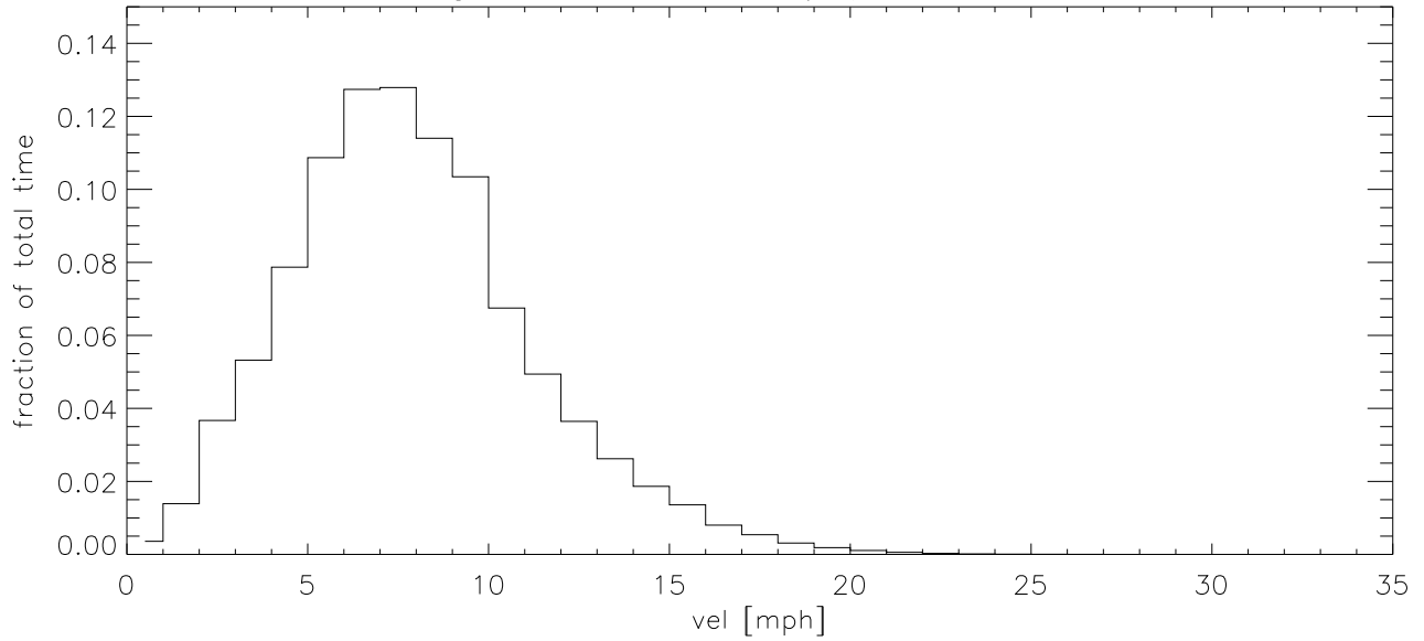
JUL18 Fraction of time wind velocity exceeds specified vel
