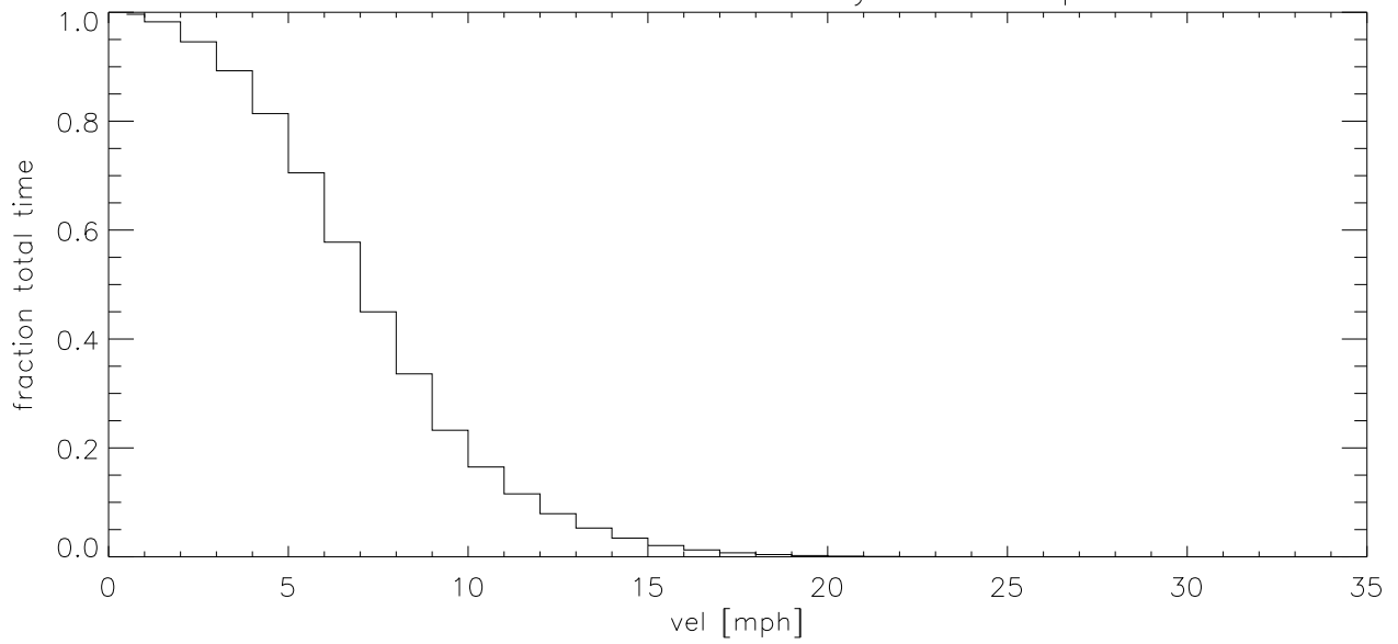
JUL18 Fraction of time wind velocity exceeds specified vel (blowup)
