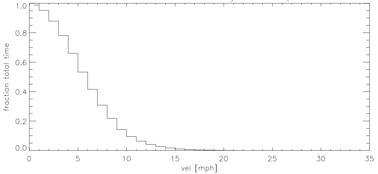
JUL17 Fraction of time wind velocity exceeds specified vel (blowup)
