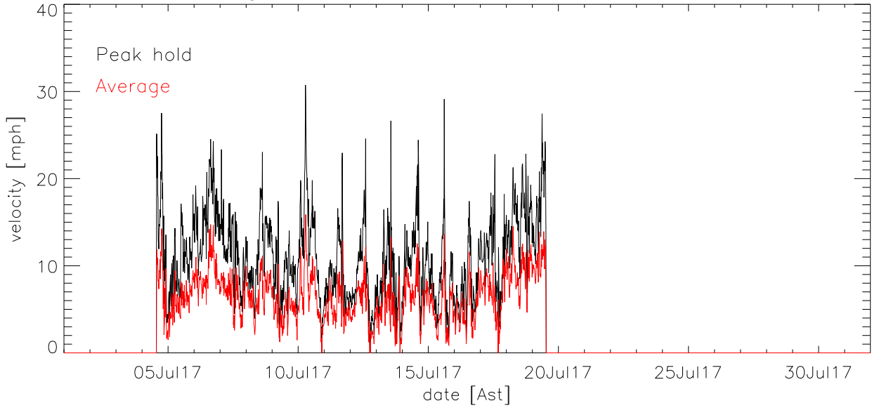
JUL17 Average, median velocity by hour of day
