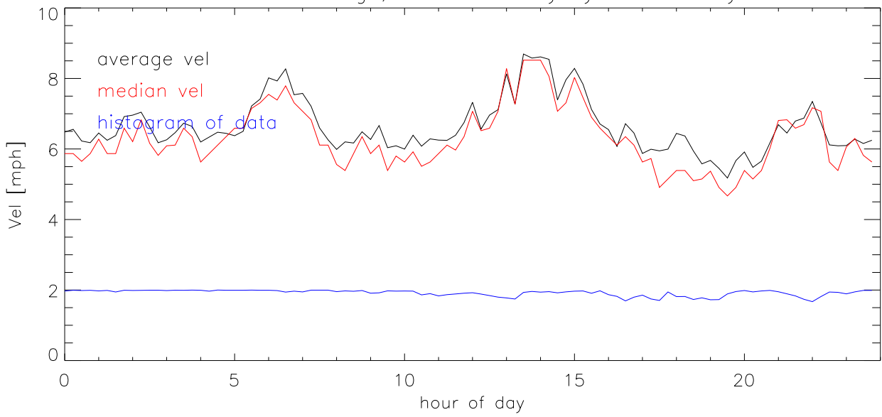
JUL17 Average, median velocity by direction
