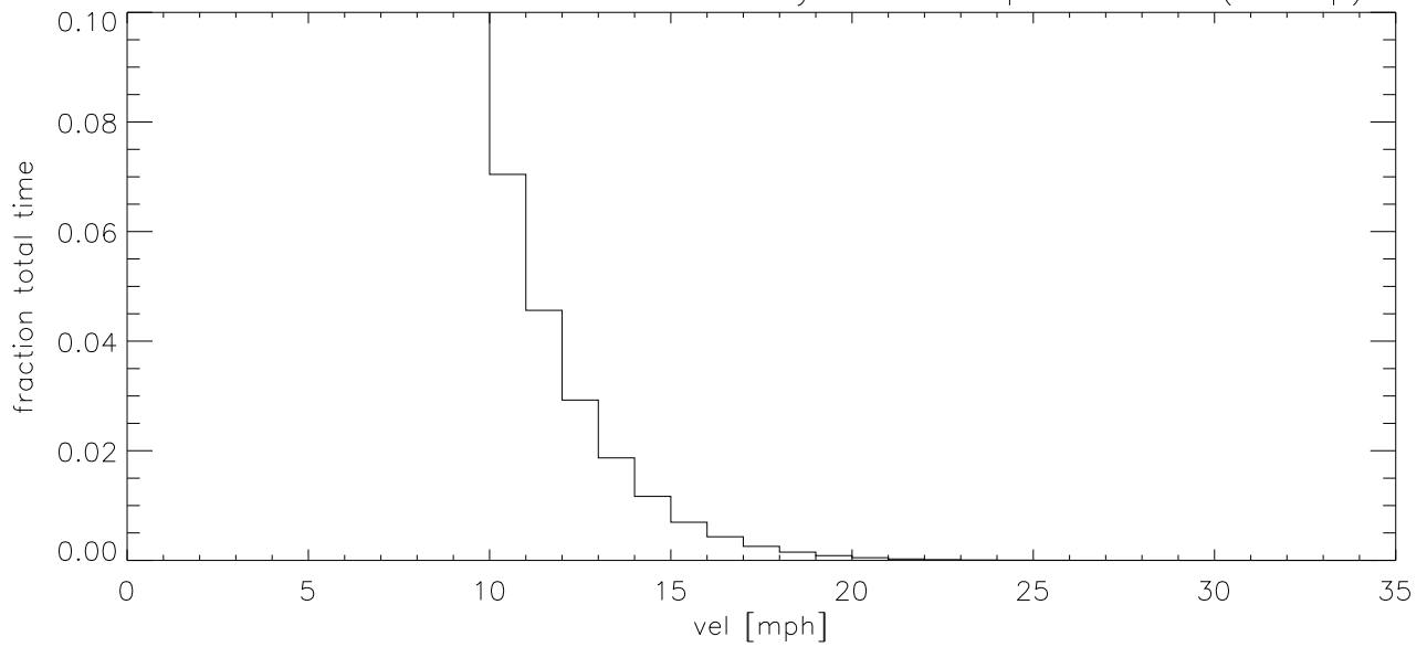
JAN16 Fraction of time wind velocity exceeds specified vel (blowup)
