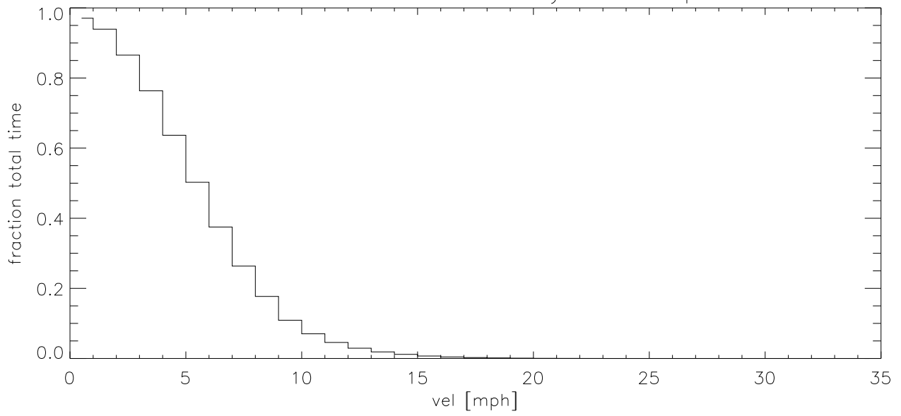
JAN16 Fraction of time wind velocity exceeds specified vel (blowup)
