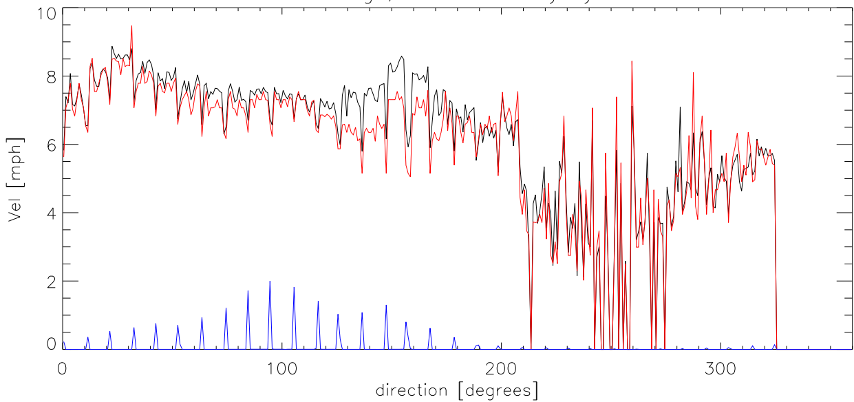
JAN16 Average, median velocity by direction
