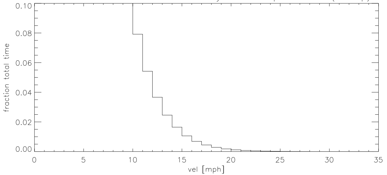
OCT15 Fraction of time wind velocity exceeds specified vel (blowup)
