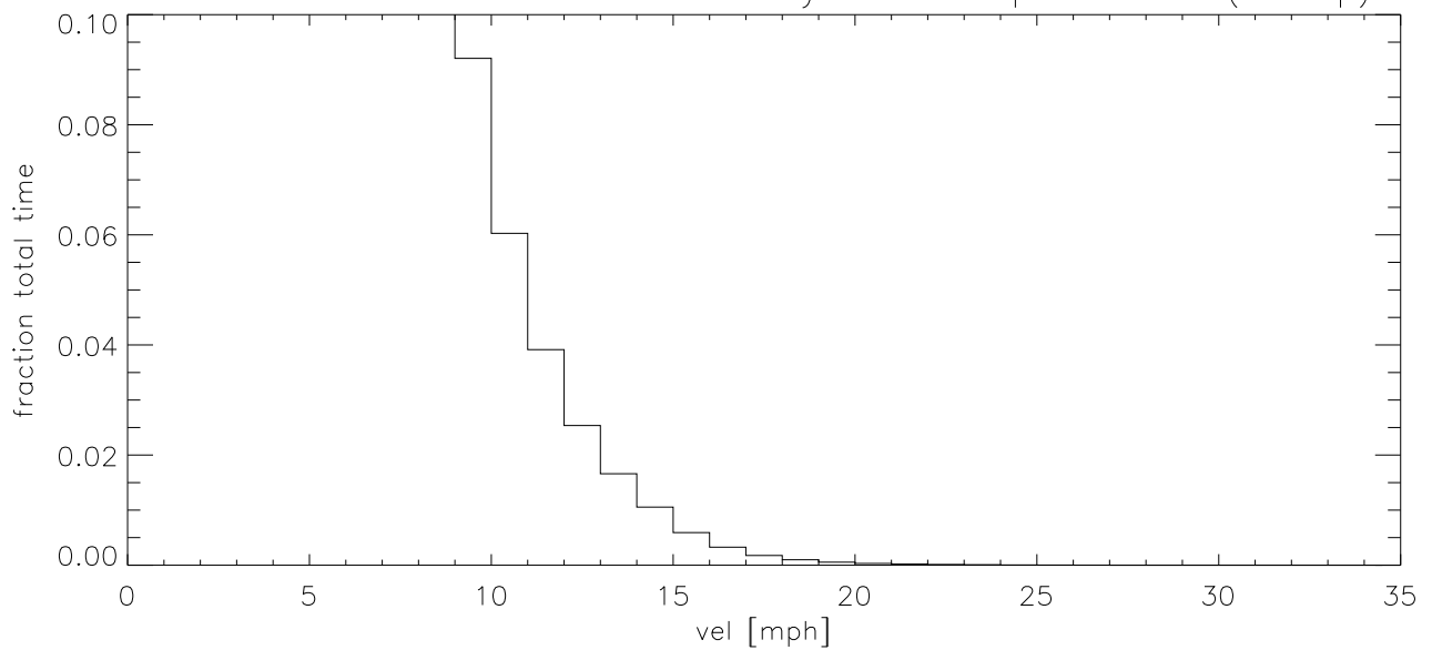
SEP15 Fraction of time wind velocity exceeds specified vel (blowup)
