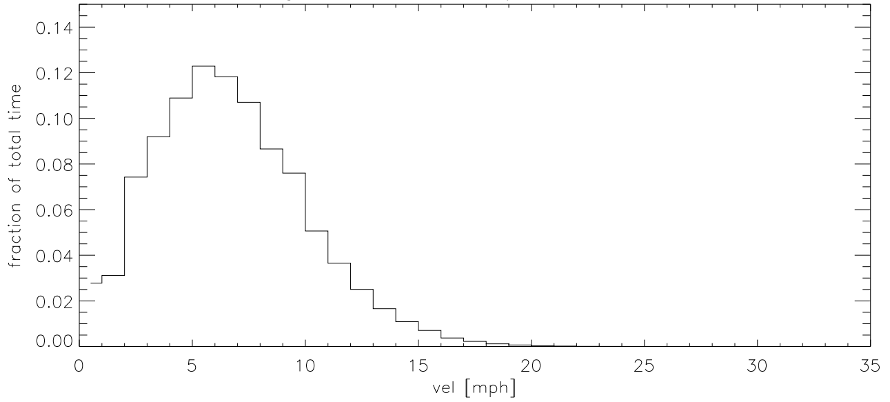
NOV14 Fraction of time wind velocity exceeds specified vel
