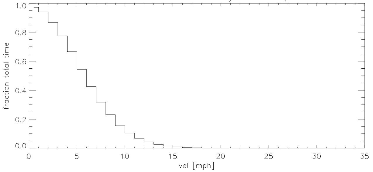
NOV14 Fraction of time wind velocity exceeds specified vel (blowup)
