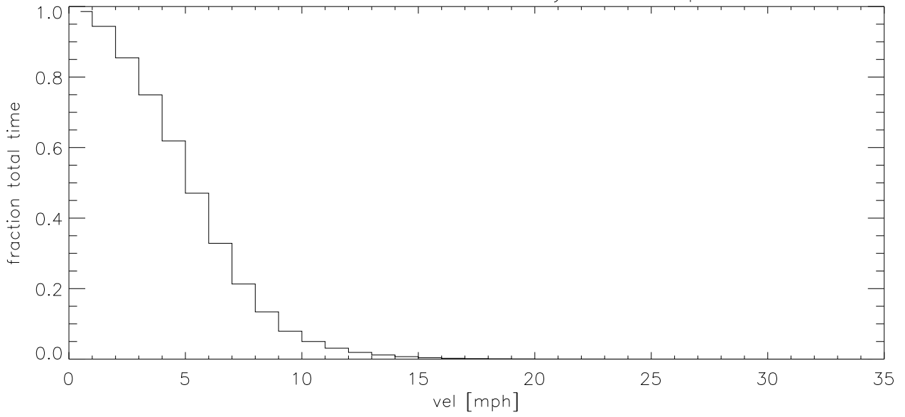
SEP14 Fraction of time wind velocity exceeds specified vel (blowup)
