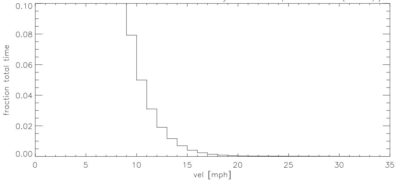
SEP14 Fraction of time wind velocity exceeds specified vel (blowup)
