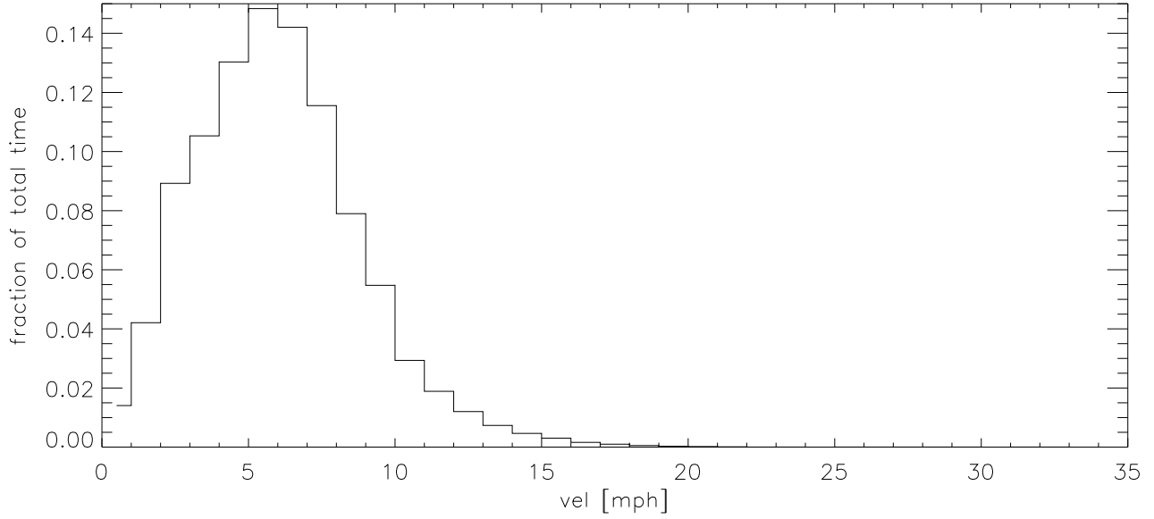
SEP14 Fraction of time wind velocity exceeds specified vel
