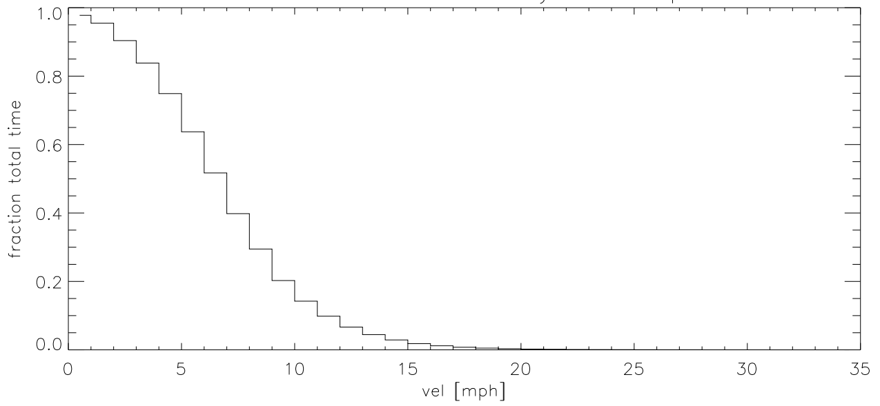
AUG14 Fraction of time wind velocity exceeds specified vel (blowup)
