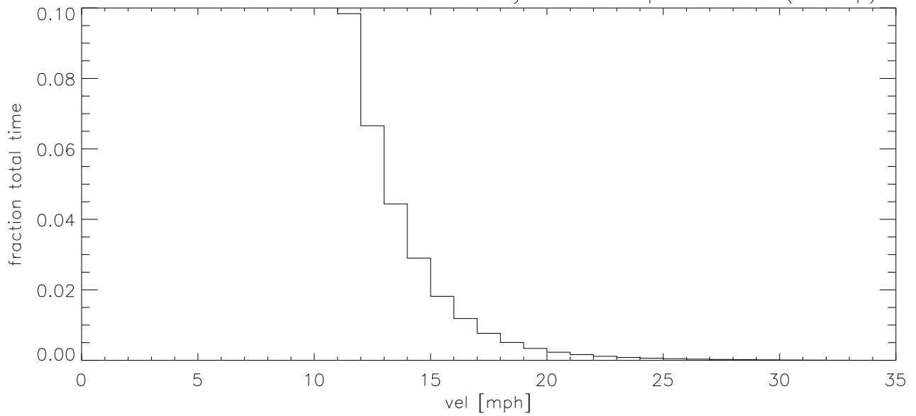
AUG14 Fraction of time wind velocity exceeds specified vel (blowup)
