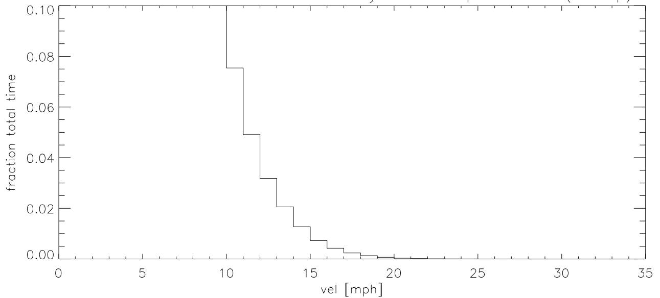
MAY14 Fraction of time wind velocity exceeds specified vel (blowup)
