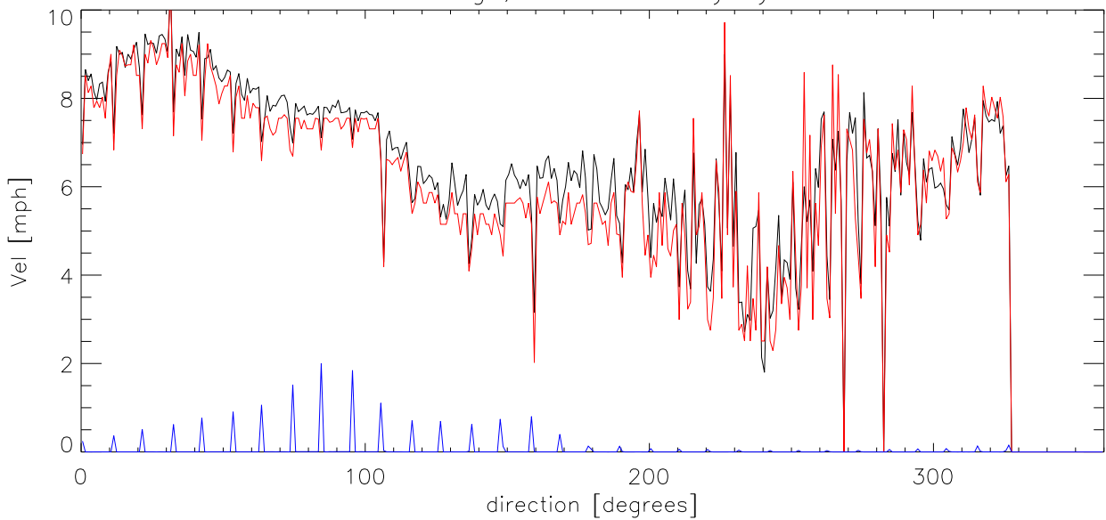
MAY14 Average, median velocity by direction
