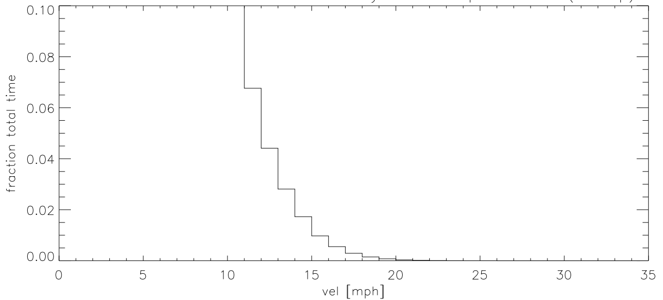
JUN13 Fraction of time wind velocity exceeds specified vel (blowup)
