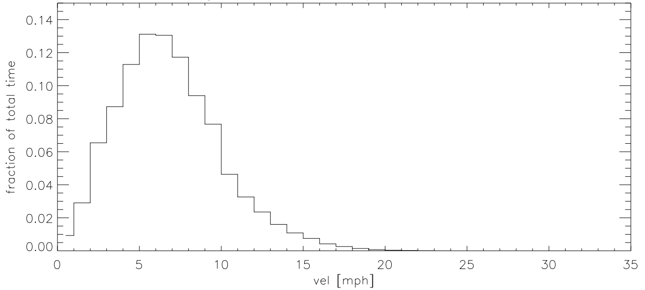
JUN13 Fraction of time wind velocity exceeds specified vel
