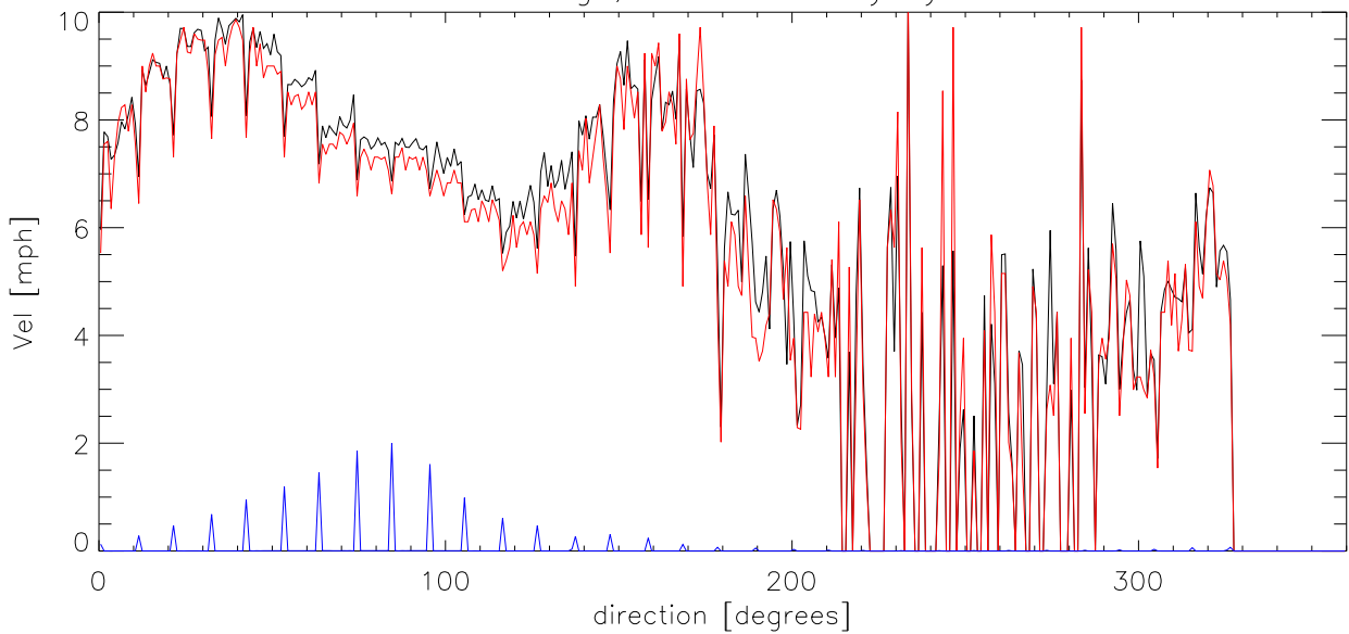
JUN13 Average, median velocity by direction
