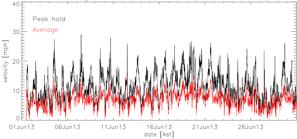
JUN13 Average, median velocity by hour of day
