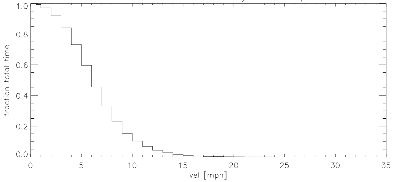
FEB12 Fraction of time wind velocity exceeds specified vel (blowup)
