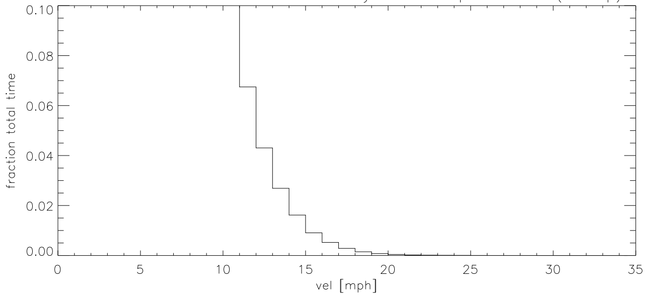
FEB12 Fraction of time wind velocity exceeds specified vel (blowup)
