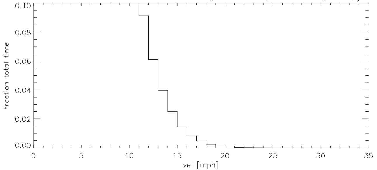
JAN12 Fraction of time wind velocity exceeds specified vel (blowup)
